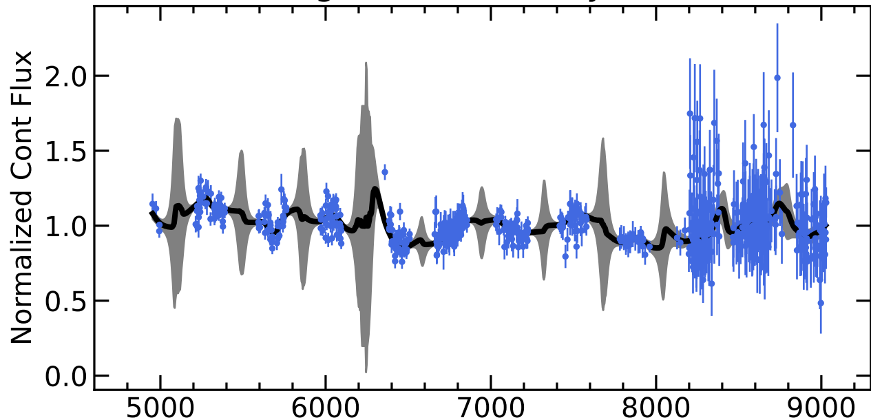
RM140 Light Curves (w/ PyROA model)
