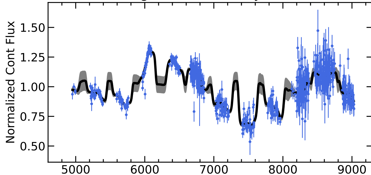
RM142 Light Curves (w/ PyROA model)
