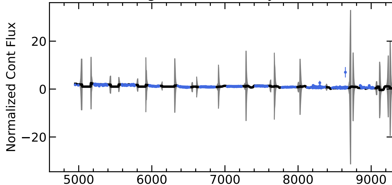
RM143 Light Curves (w/ PyROA model)
