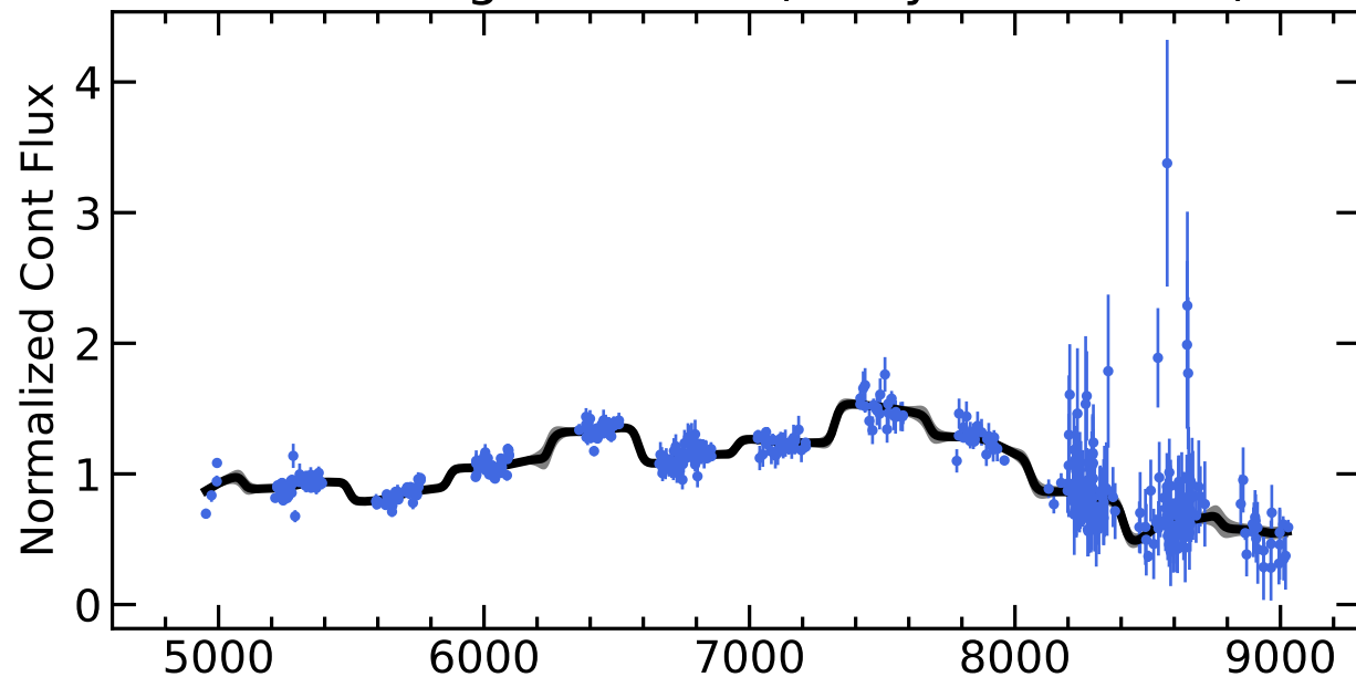
RM144 Light Curves (w/ PyROA model)
