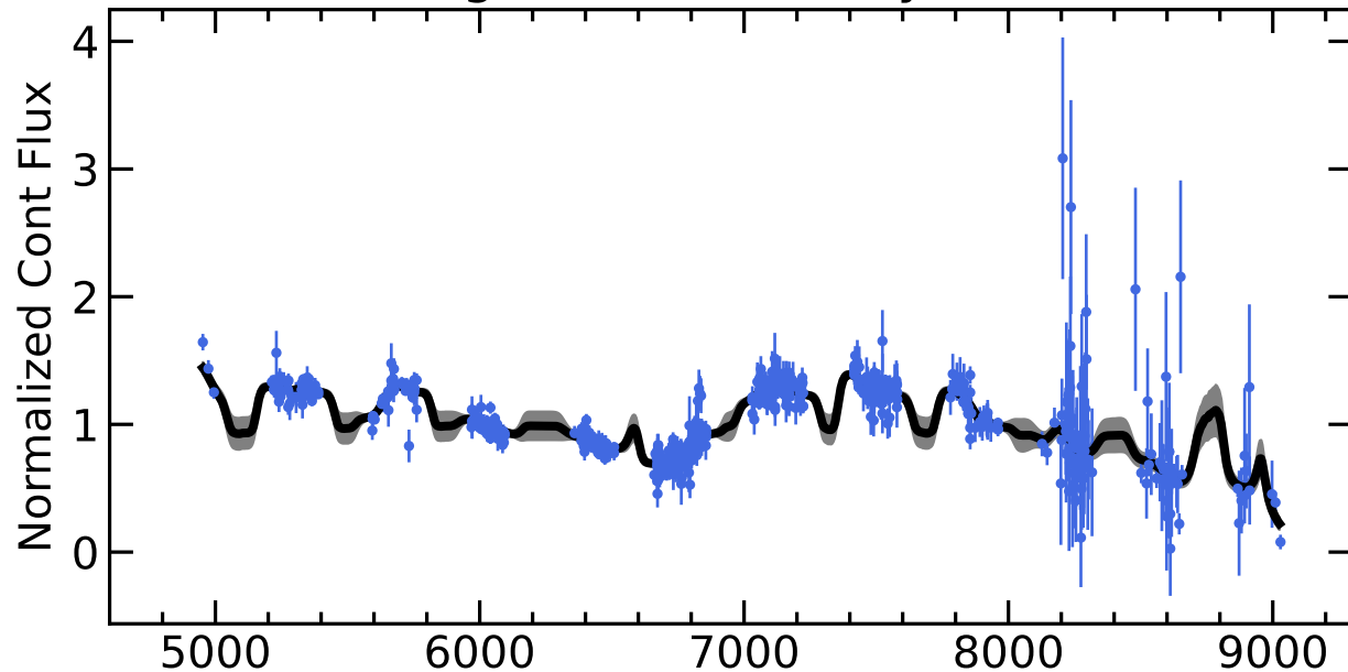
RM145 Light Curves (w/ PyROA model)
