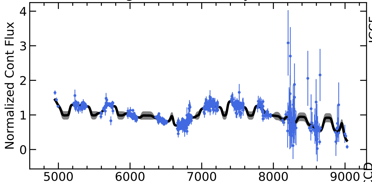
RM145 Light Curves (w/ PyROA model)
