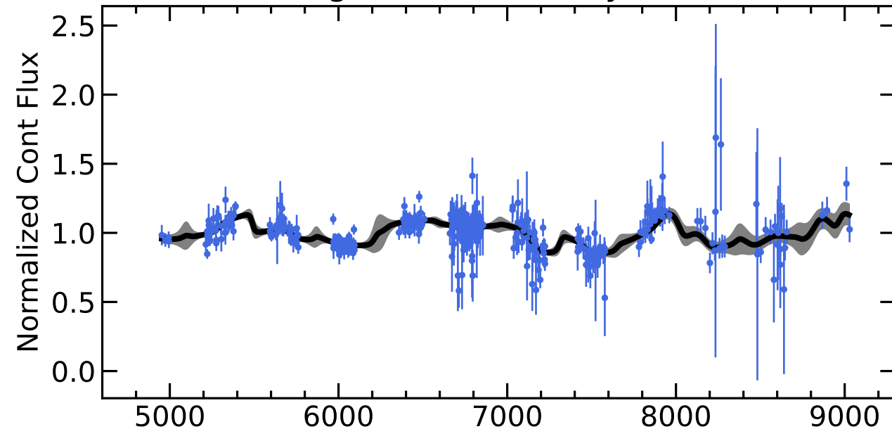
RM148 Light Curves (w/ PyROA model)
