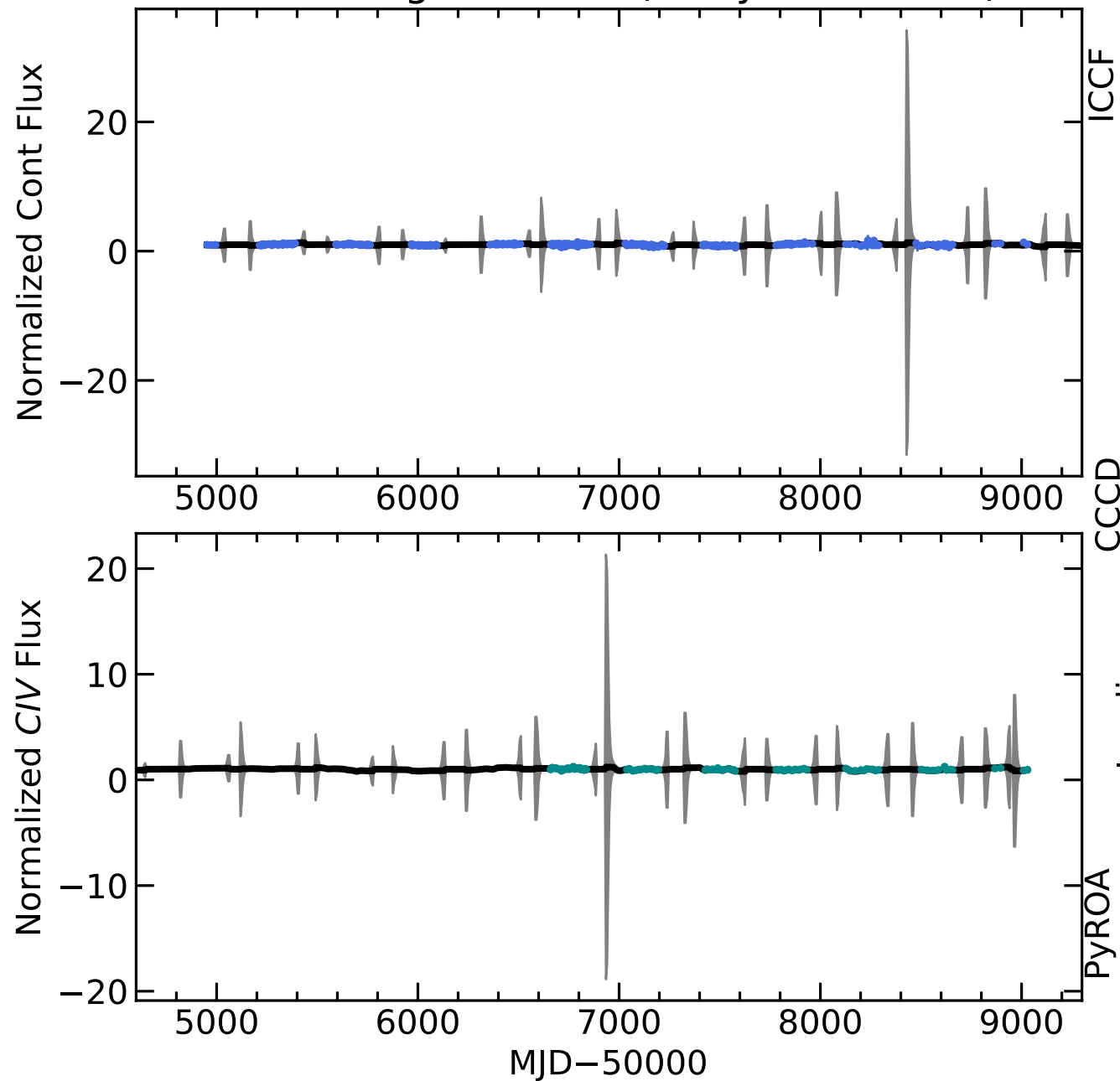
RM148 Light Curves (w/ PyROA model)
