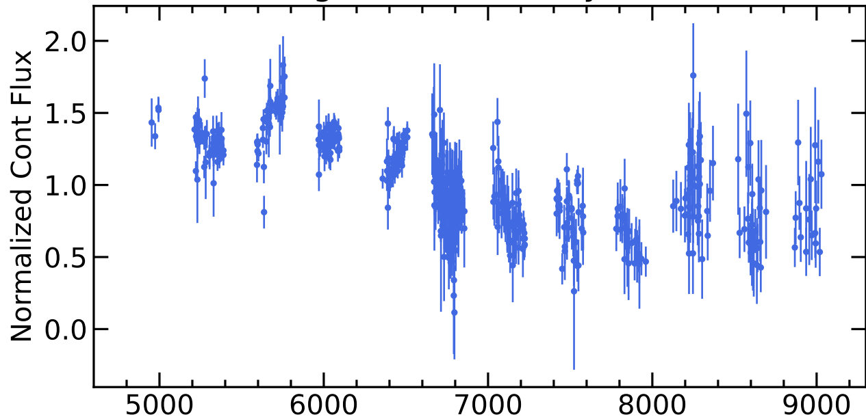
RM149 Light Curves (w/ PyROA model)
