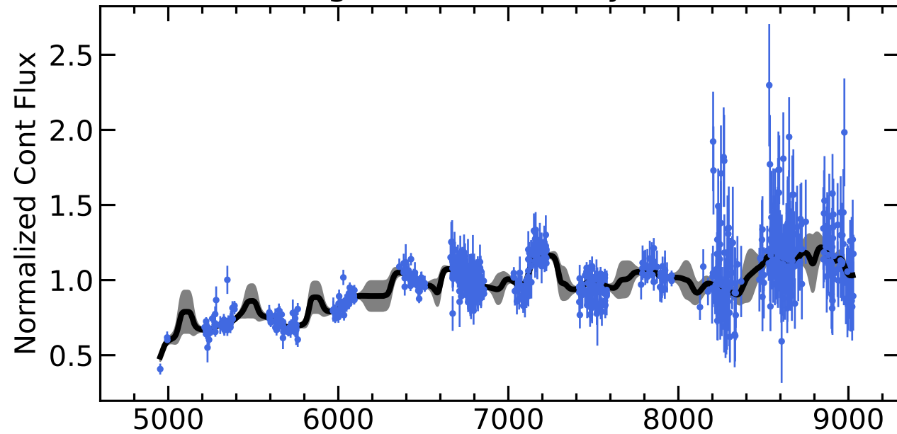
RM150 Light Curves (w/ PyROA model)
