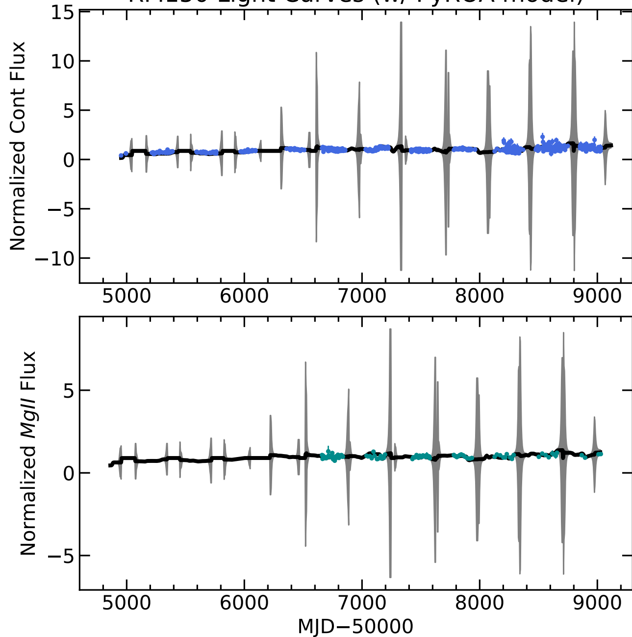
RM150 Light Curves (w/ PyROA model)
