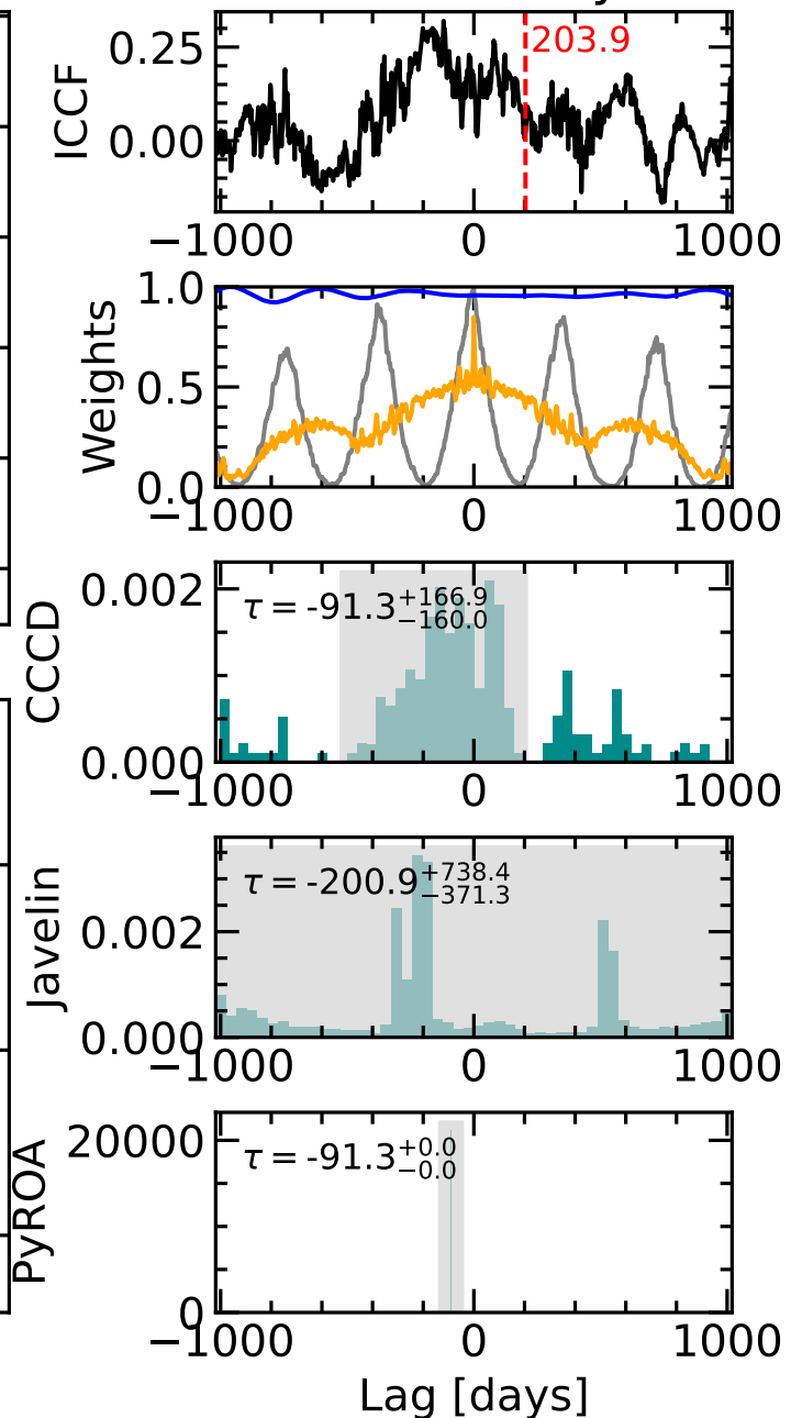
Time Delay
