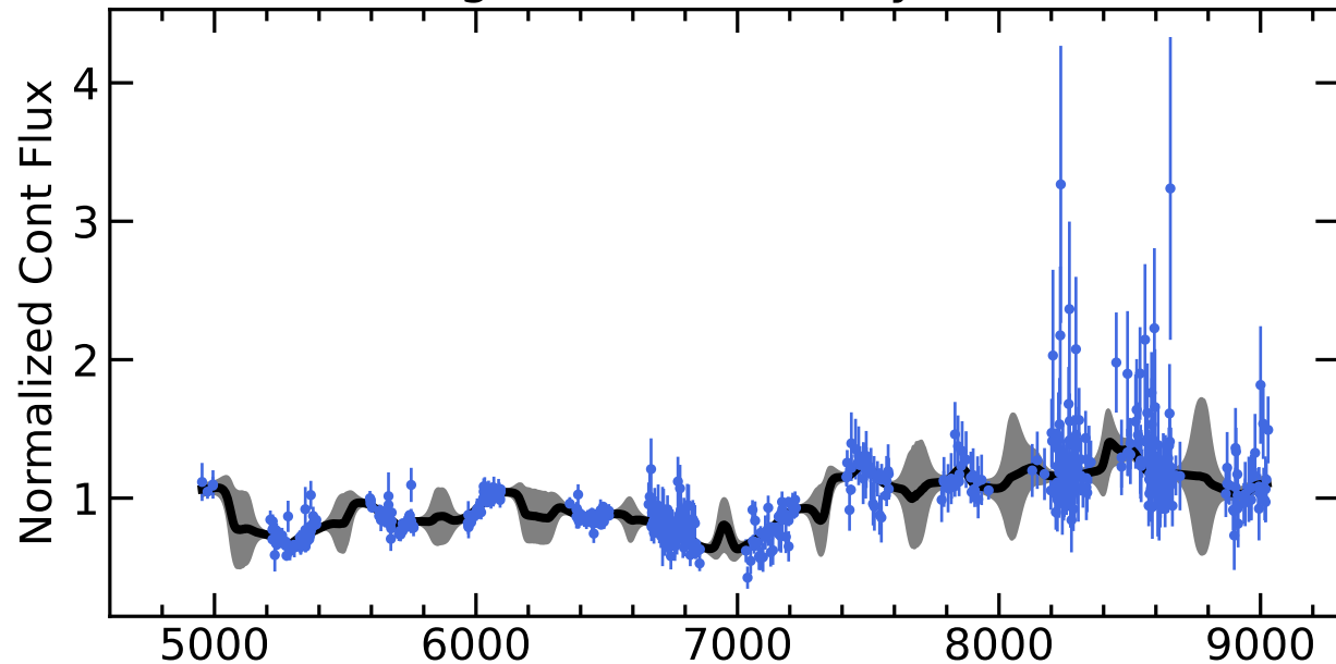
RM151 Light Curves (w/ PyROA model)
