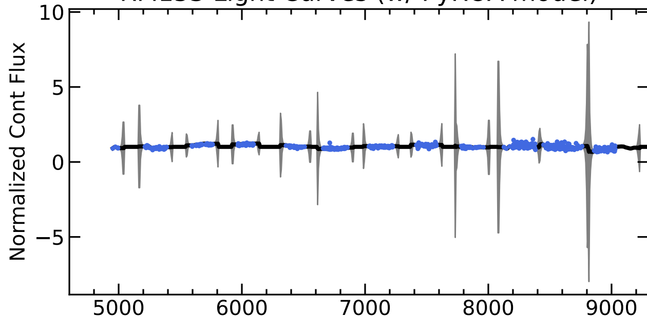
RM153 Light Curves (w/ PyROA model)
