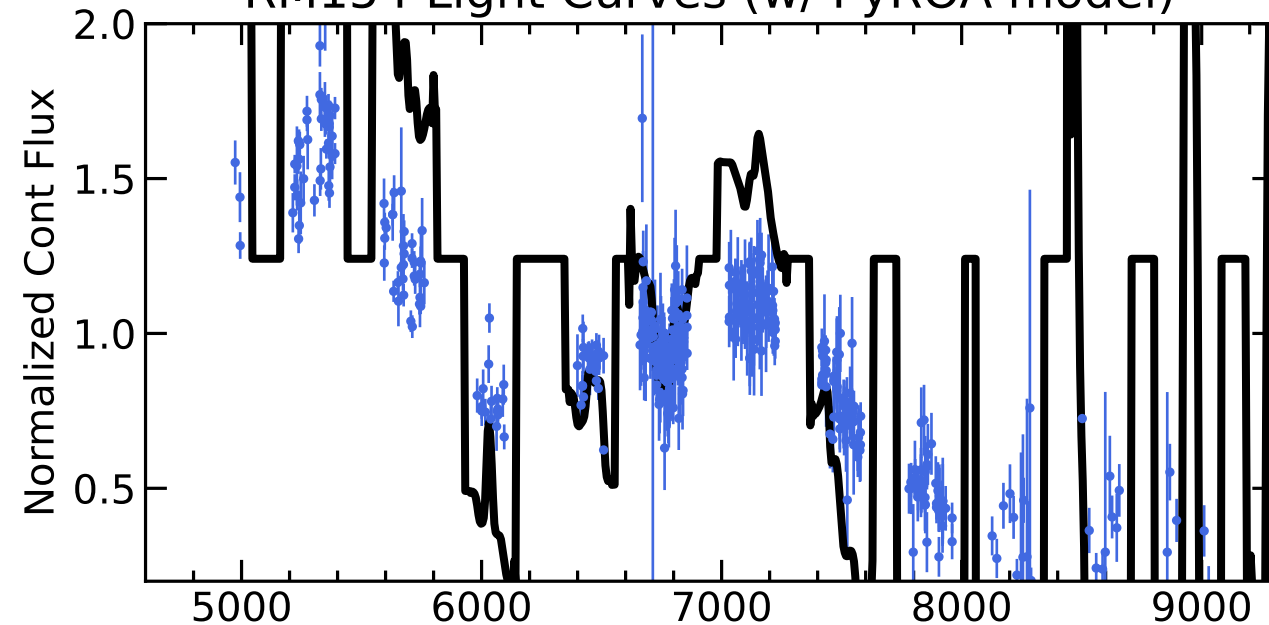
RM154 Light Curves (w/ PyROA model)
