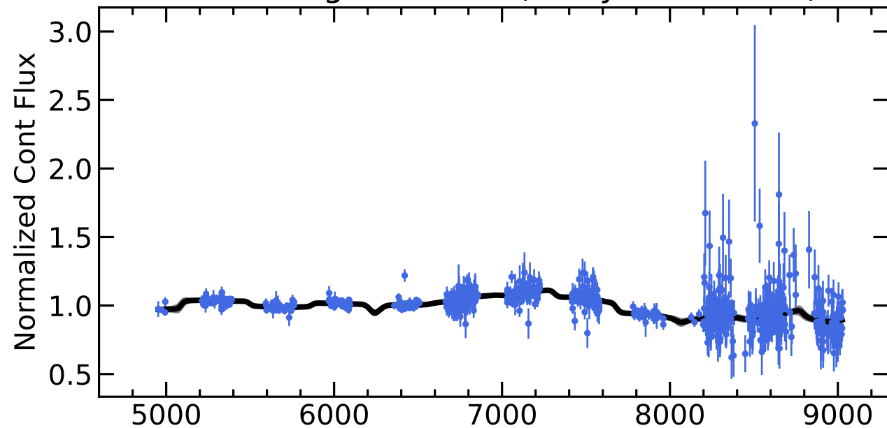
RM155 Light Curves (w/ PyROA model)
