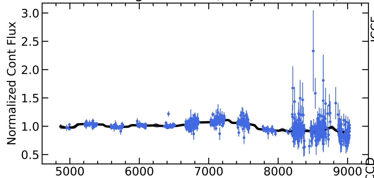
RM155 Light Curves (w/ PyROA model)
