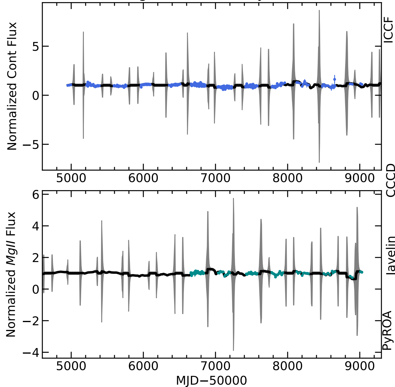
RM156 Light Curves (w/ PyROA model)
