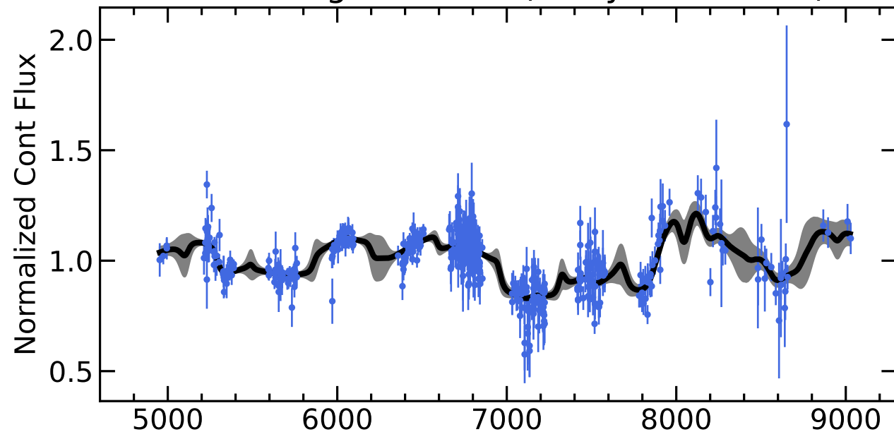
RM156 Light Curves (w/ PyROA model)
