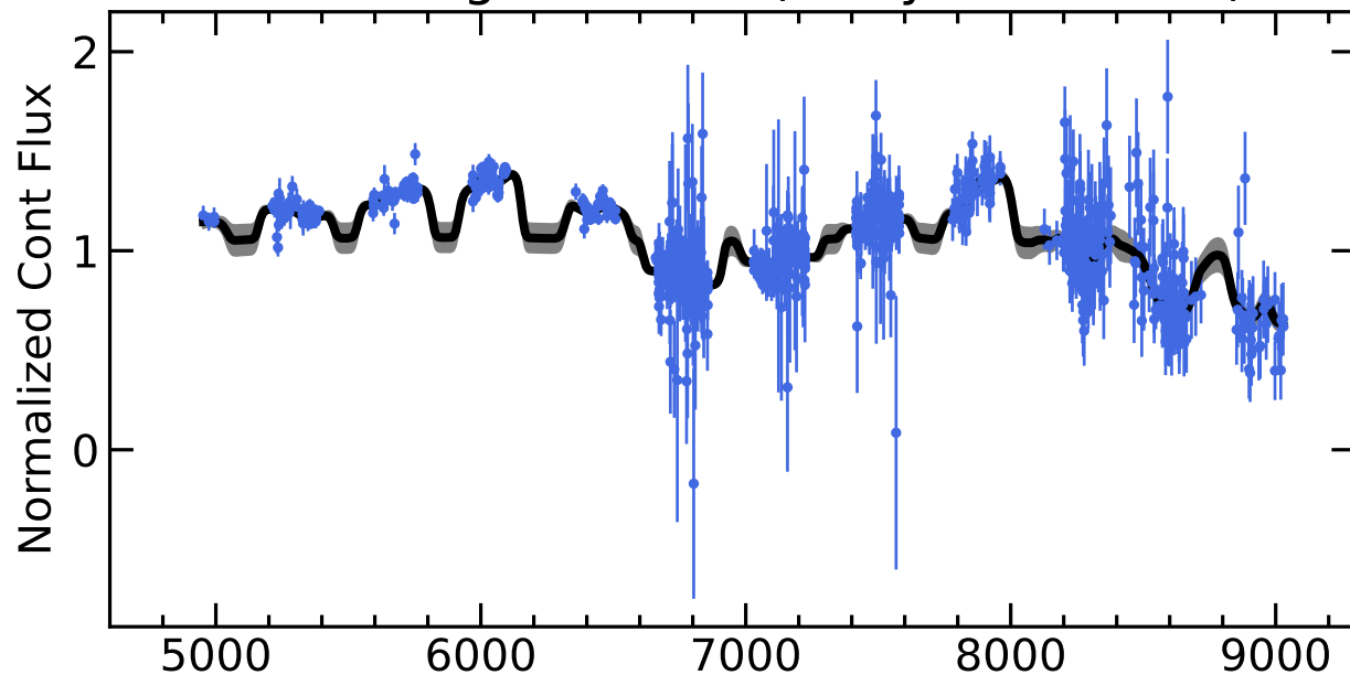
RM158 Light Curves (w/ PyROA model)
