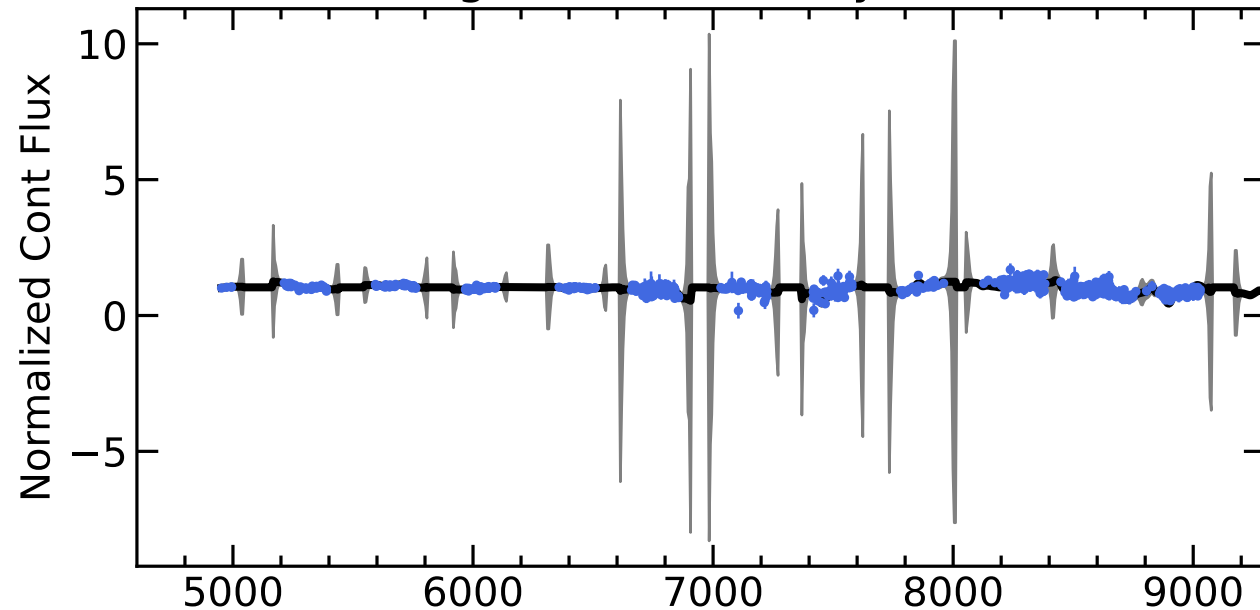
RM159 Light Curves (w/ PyROA model)
