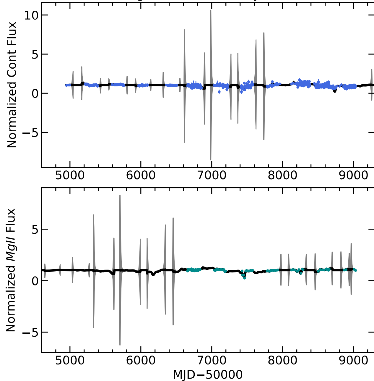
RM159 Light Curves (w/ PyROA model)
