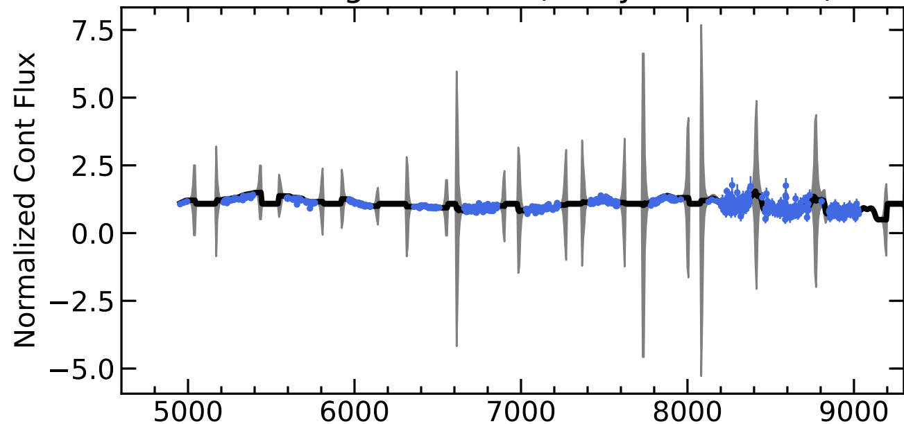
RM161 Light Curves (w/ PyROA model)
