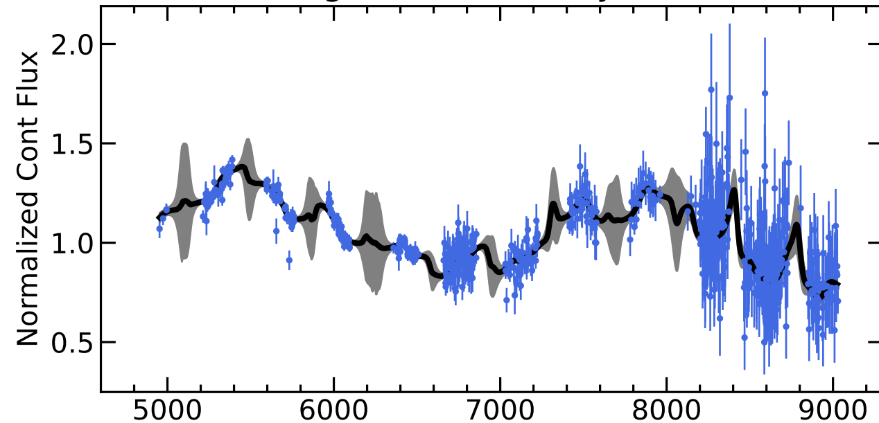
RM161 Light Curves (w/ PyROA model)
