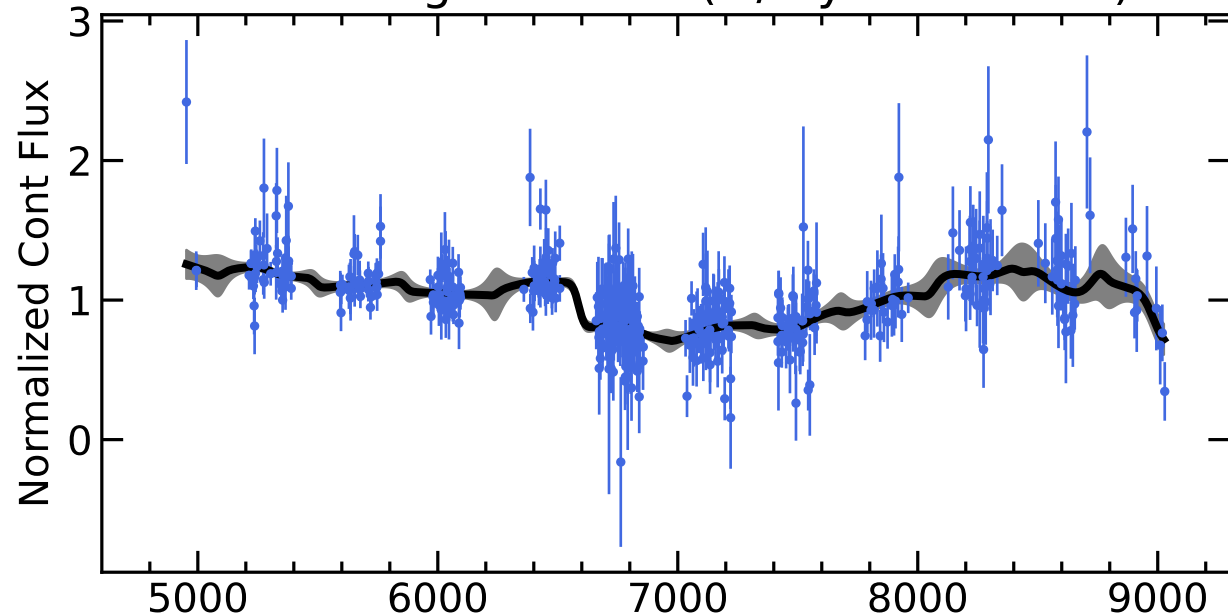
RM162 Light Curves (w/ PyROA model)
