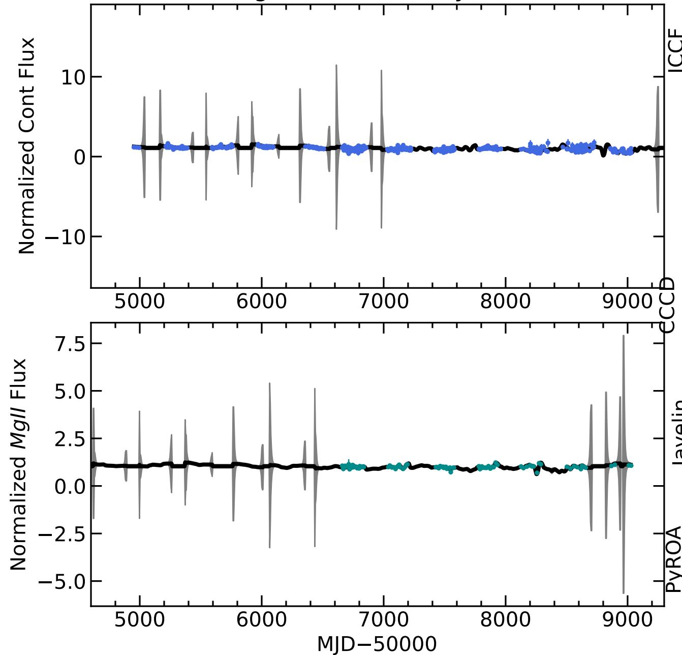
RM163 Light Curves (w/ PyROA model)
