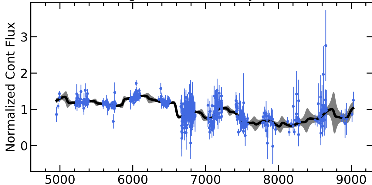
RM167 Light Curves (w/ PyROA model)
