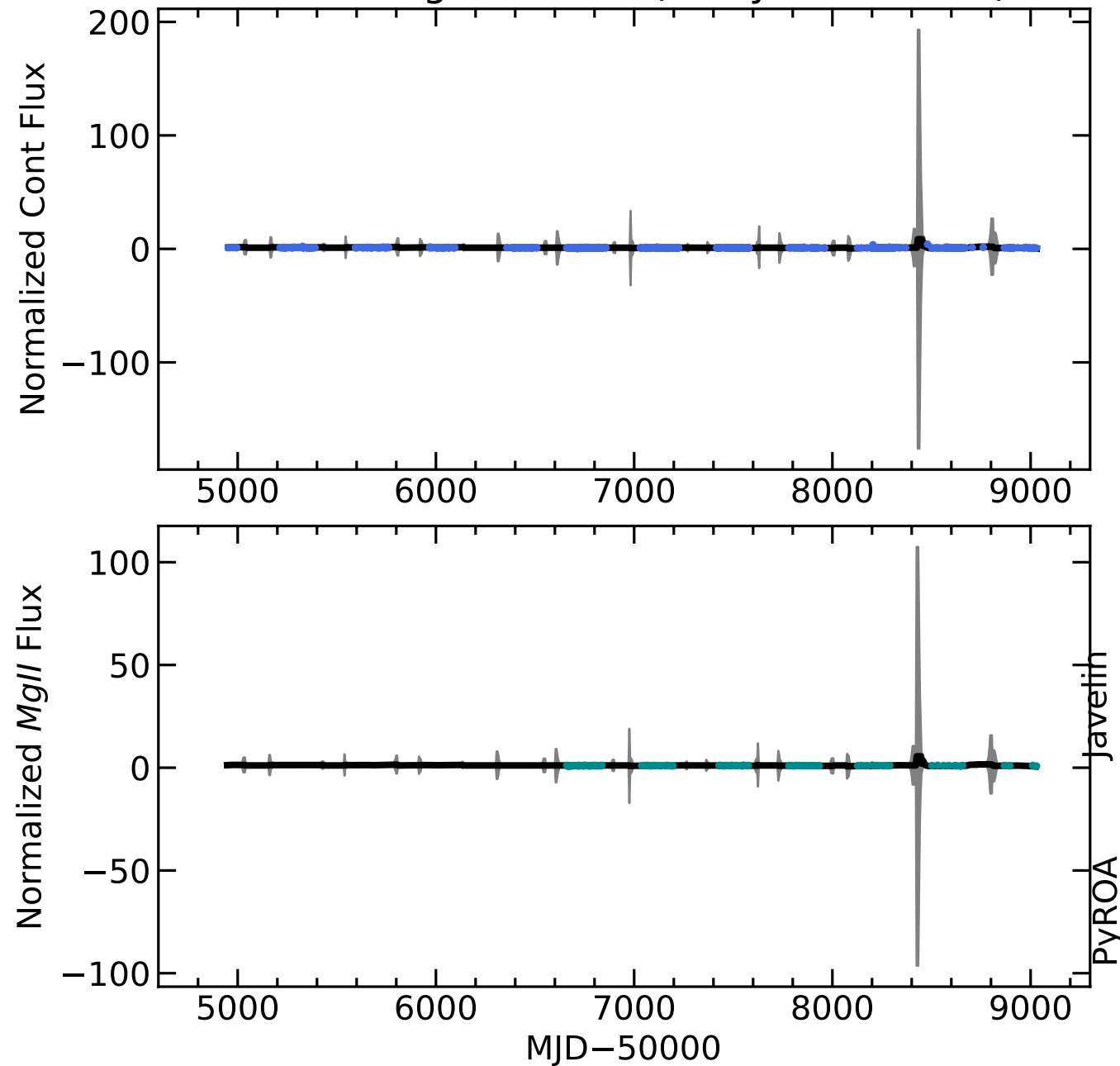
RM168 Light Curves (w/ PyROA model)
