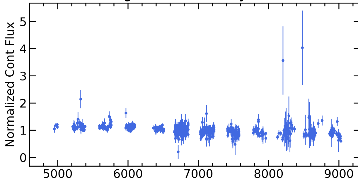
RM168 Light Curves (w/ PyROA model)
