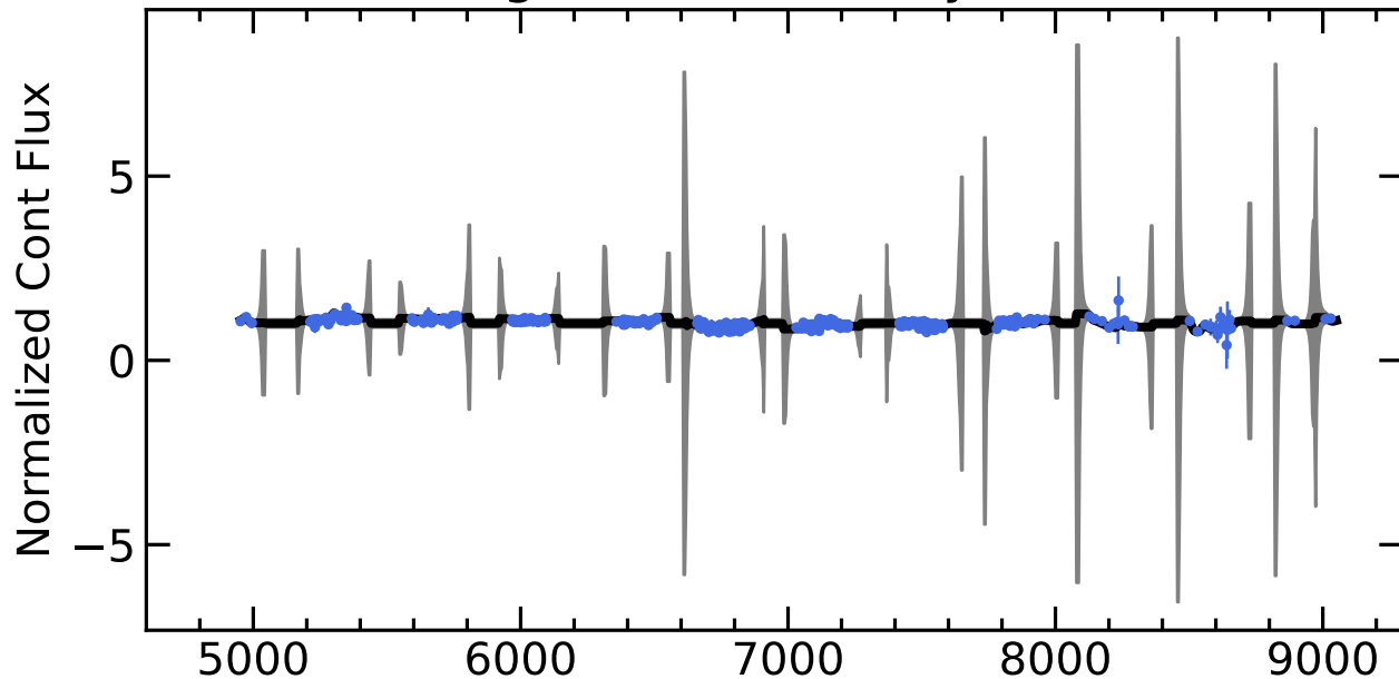
RM171 Light Curves (w/ PyROA model)
