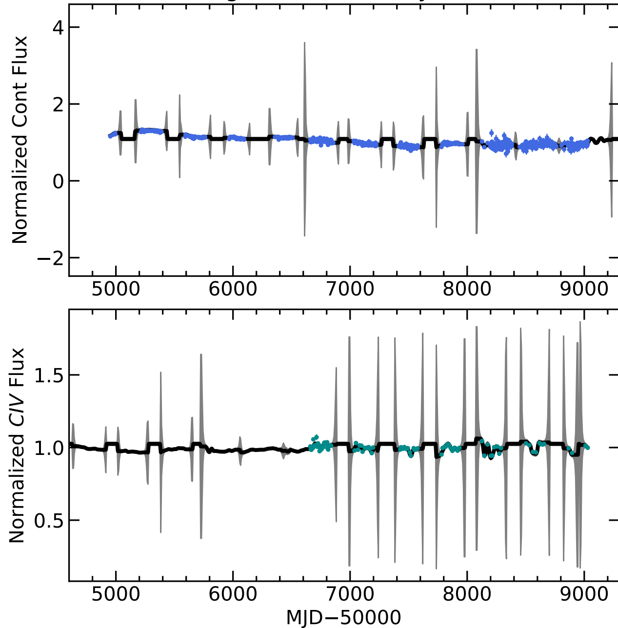
RM172 Light Curves (w/ PyROA model)
