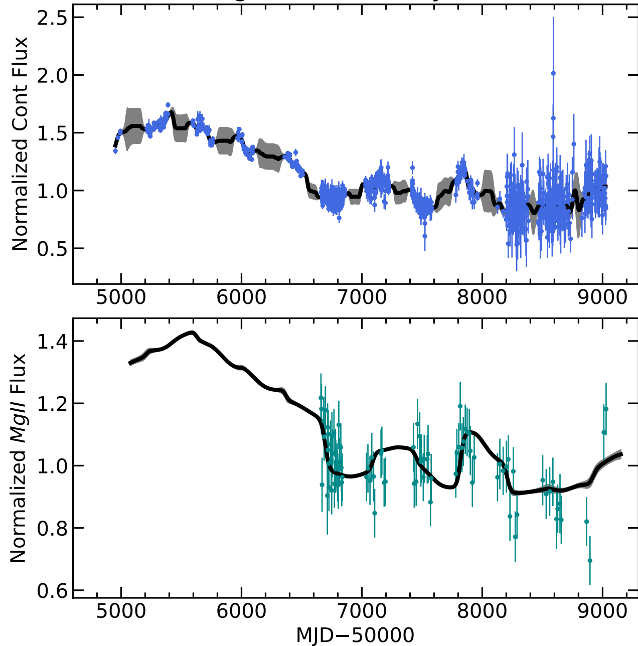
RM173 Light Curves (w/ PyROA model)
