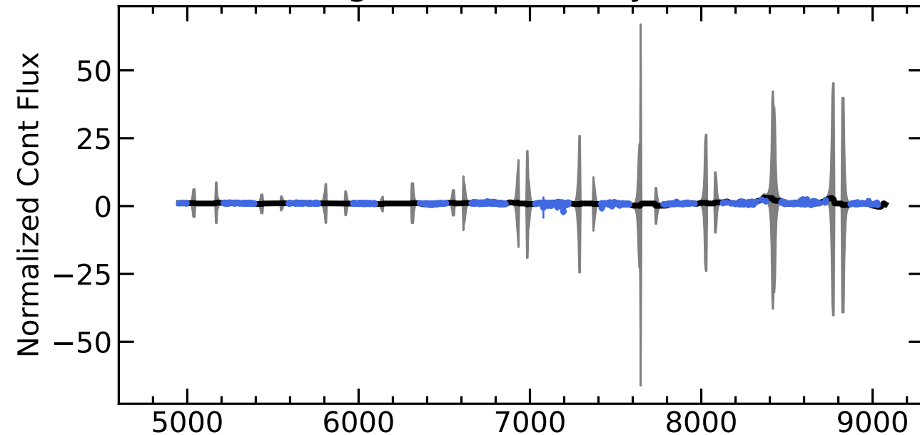
RM175 Light Curves (w/ PyROA model)
