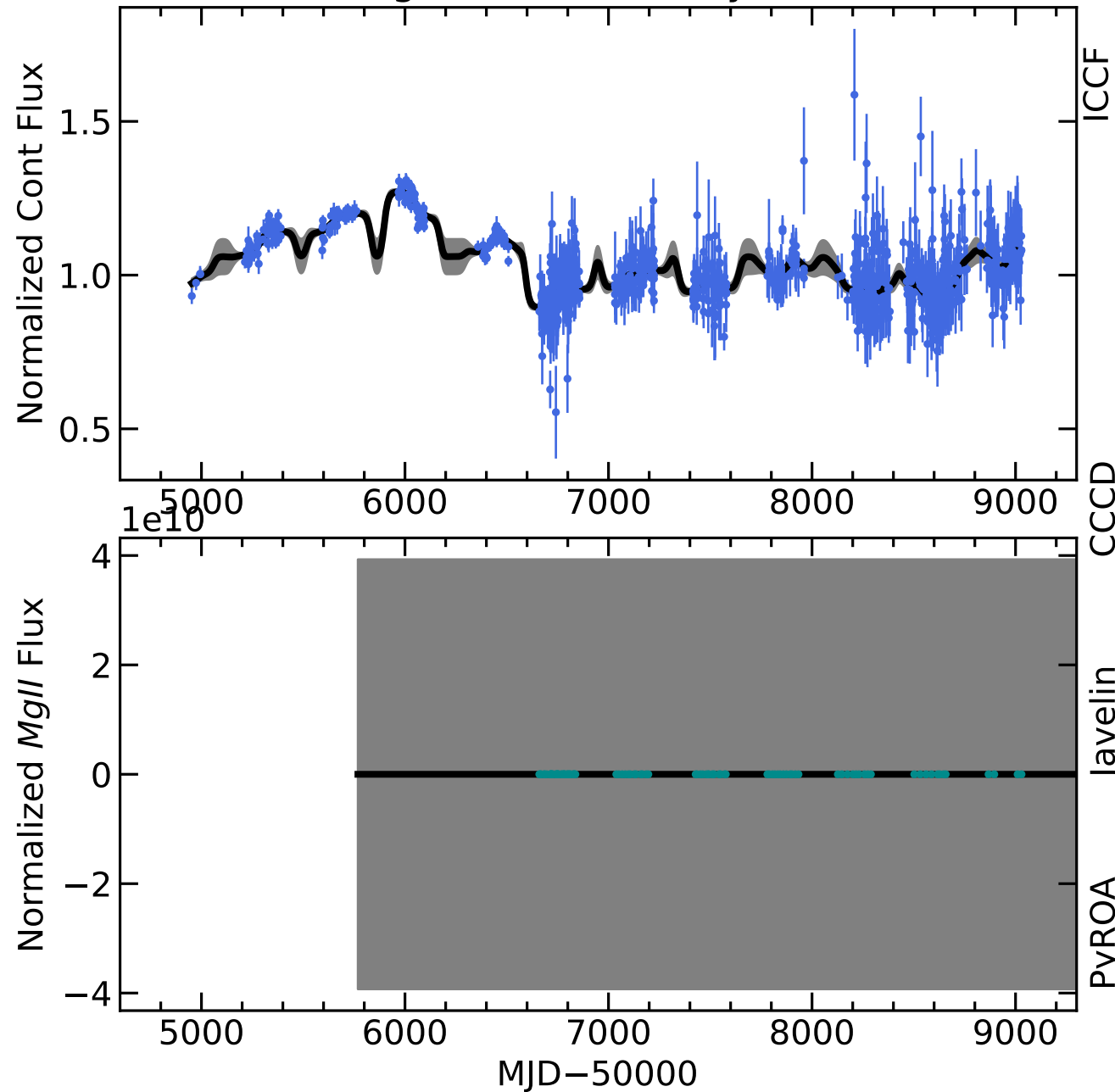
RM176 Light Curves (w/ PyROA model)
