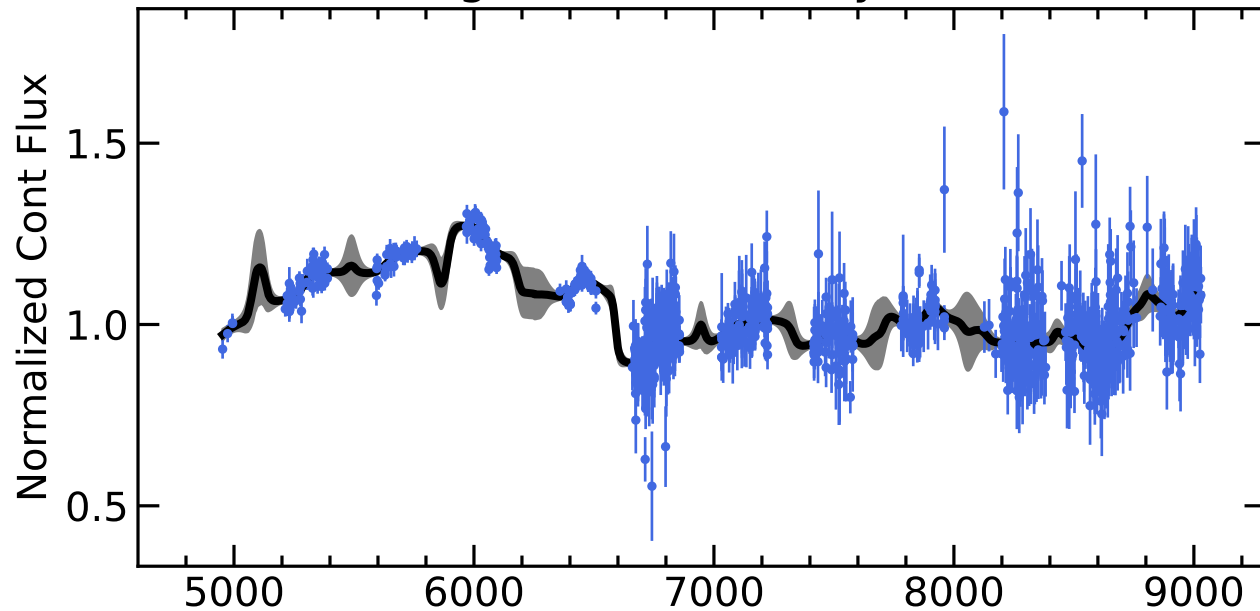
RM176 Light Curves (w/ PyROA model)
