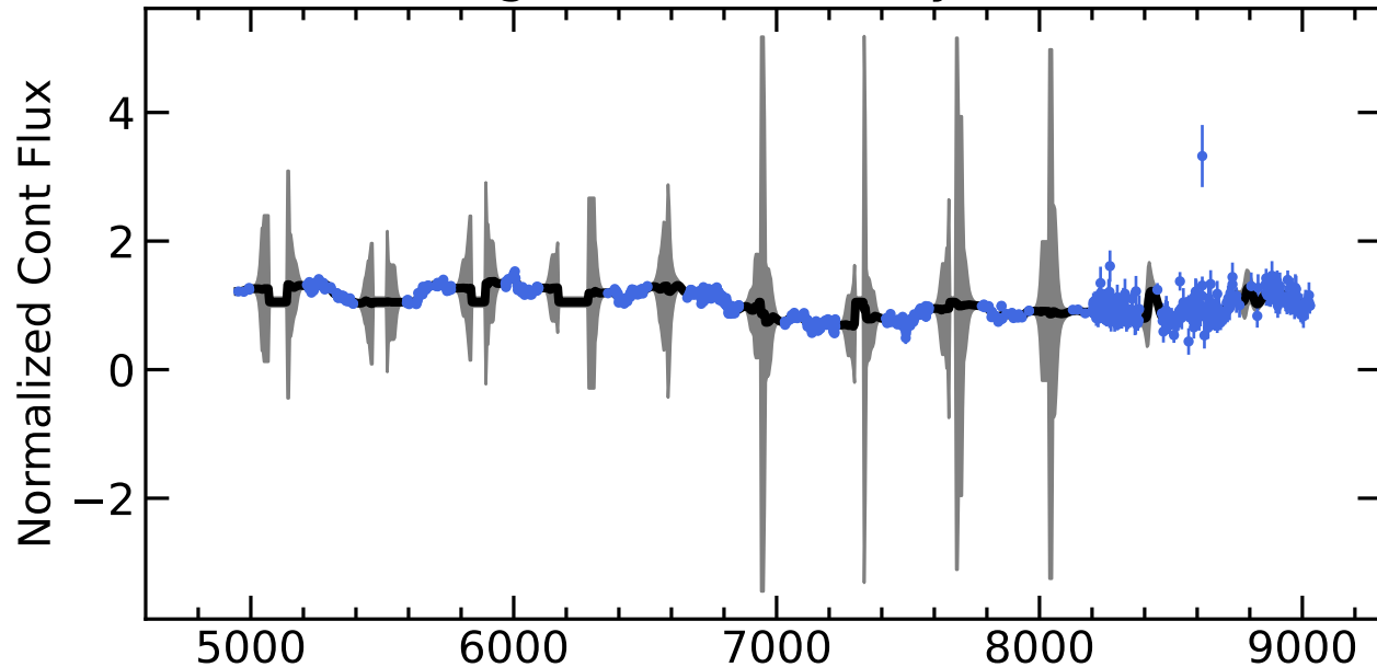
RM177 Light Curves (w/ PyROA model)
