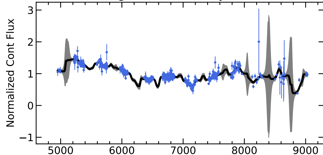
RM179 Light Curves (w/ PyROA model)
