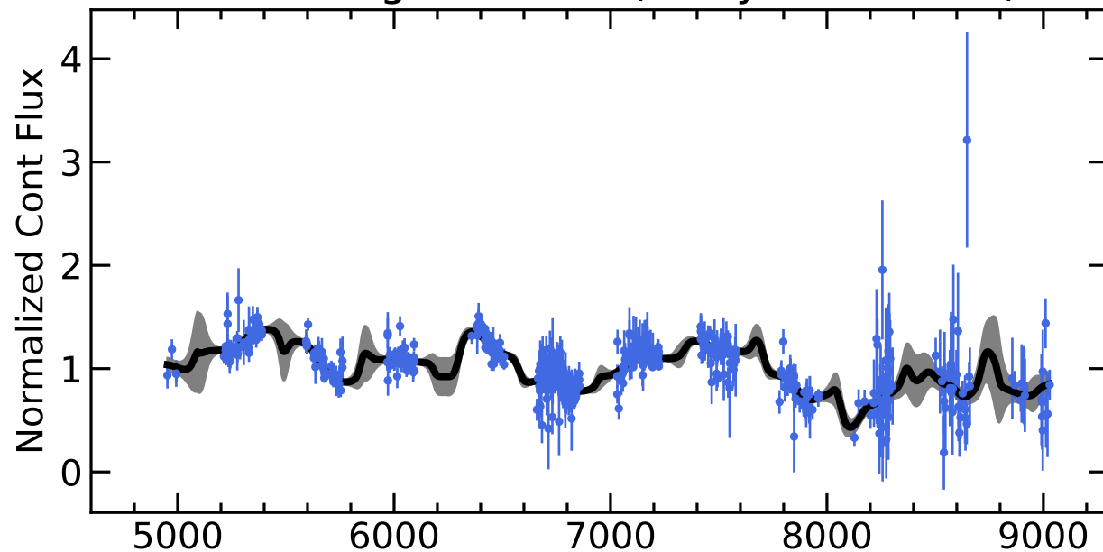
RM181 Light Curves (w/ PyROA model)
