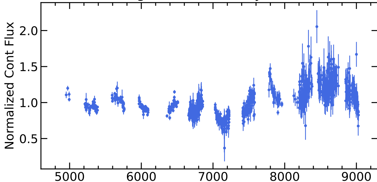
RM182 Light Curves (w/ PyROA model)
