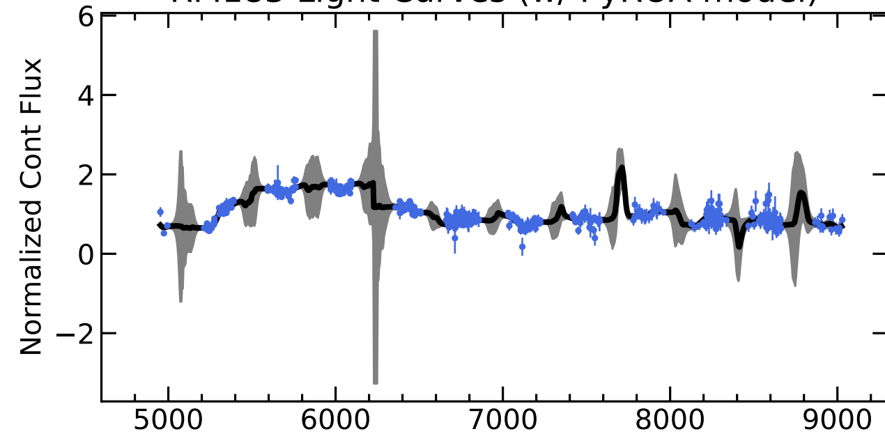
RM183 Light Curves (w/ PyROA model)
