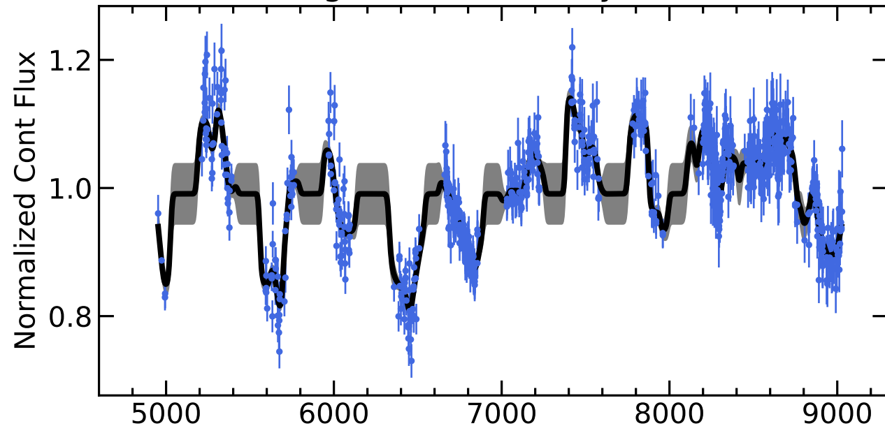
RM184 Light Curves (w/ PyROA model)
