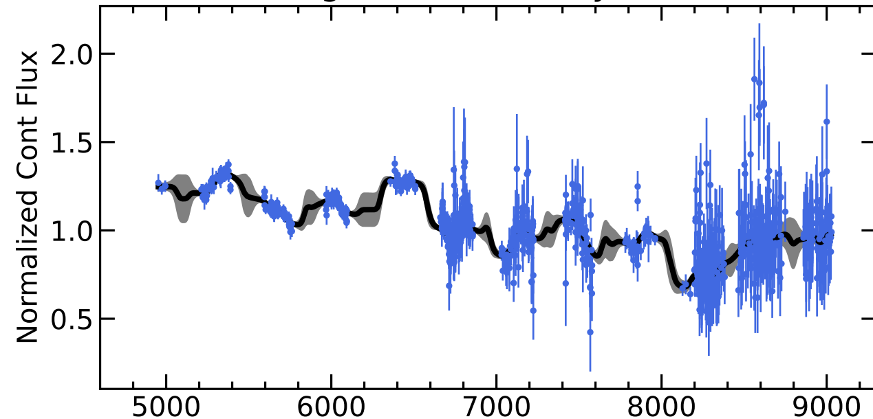
RM185 Light Curves (w/ PyROA model)
