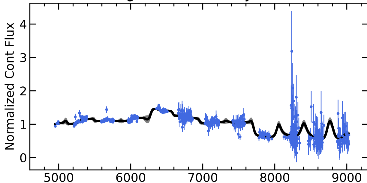
RM186 Light Curves (w/ PyROA model)
