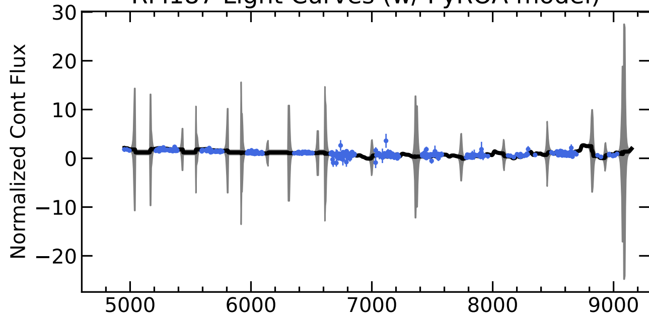
RM187 Light Curves (w/ PyROA model)
