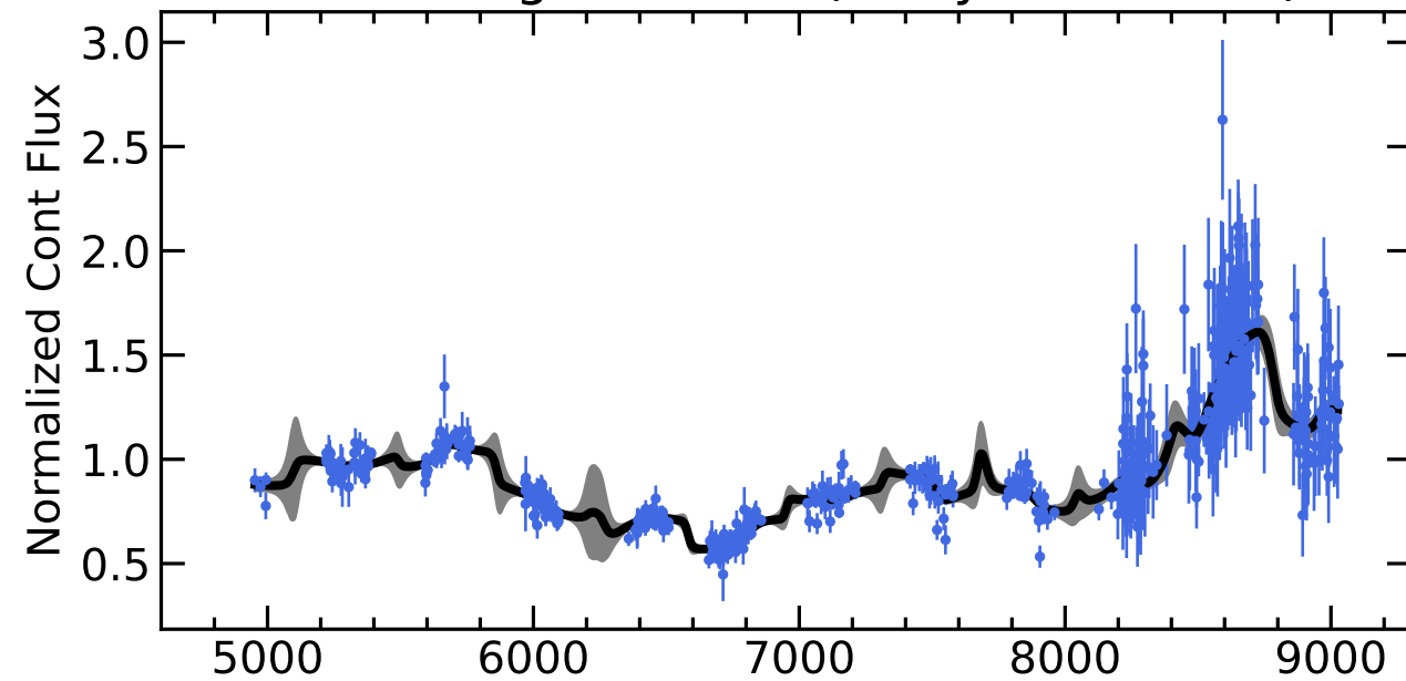
RM188 Light Curves (w/ PyROA model)
