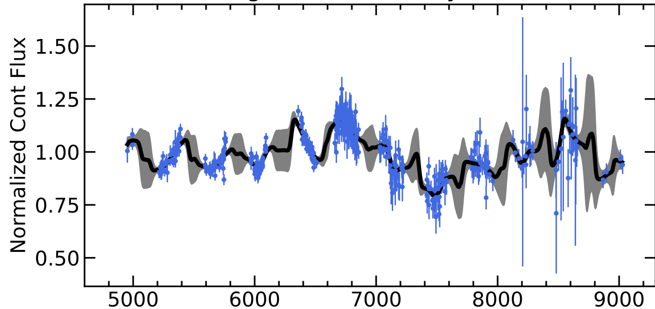
RM189 Light Curves (w/ PyROA model)
