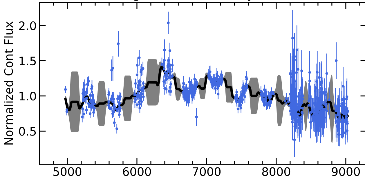
RM191 Light Curves (w/ PyROA model)
