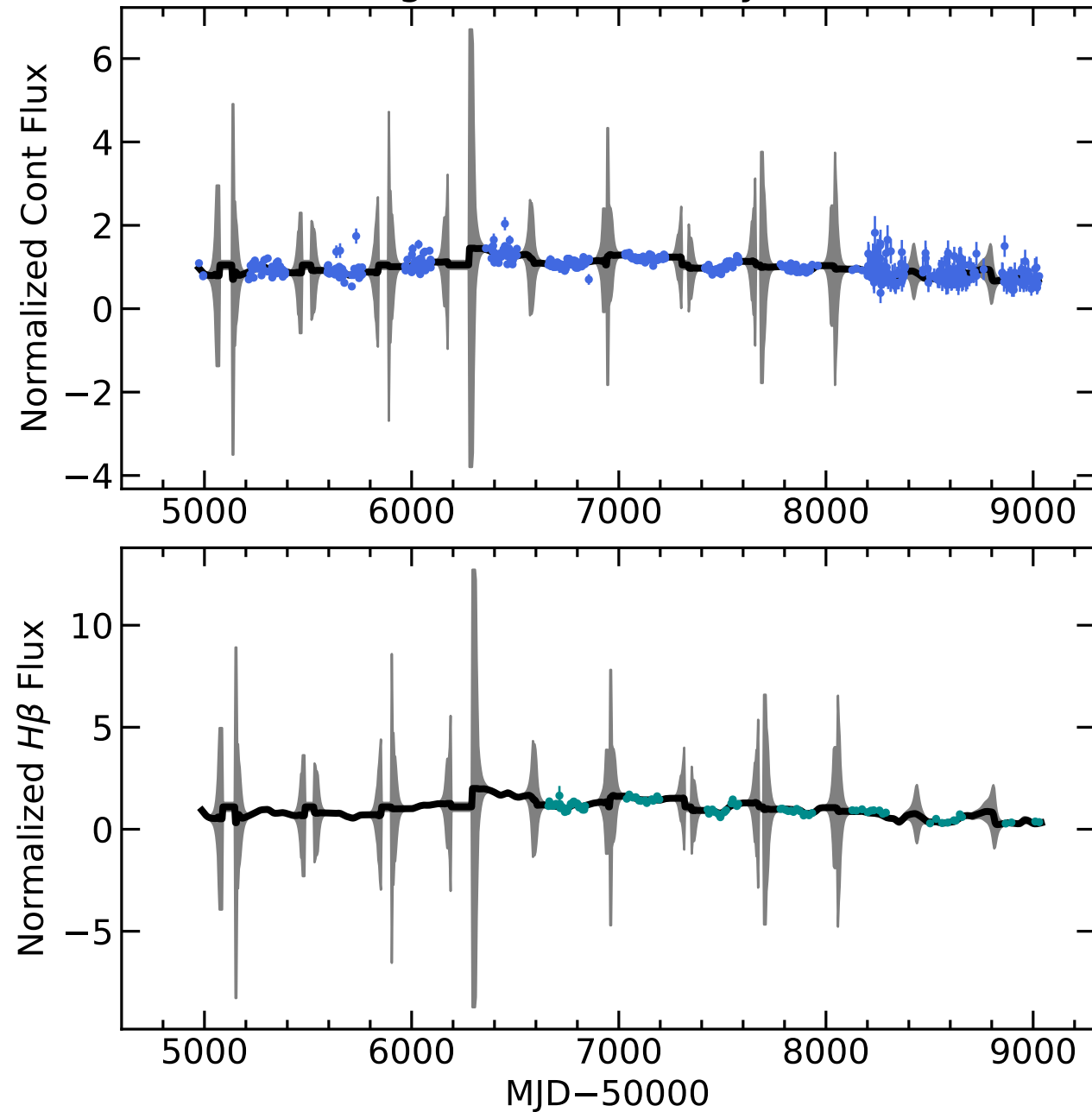
RM191 Light Curves (w/ PyROA model)
