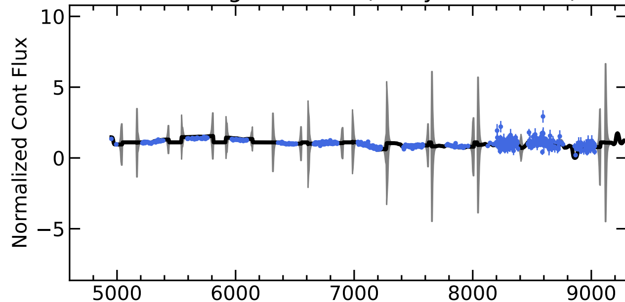
RM192 Light Curves (w/ PyROA model)
