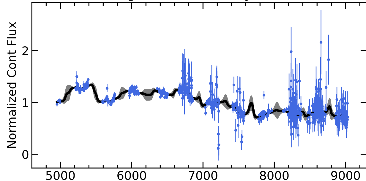
RM193 Light Curves (w/ PyROA model)
