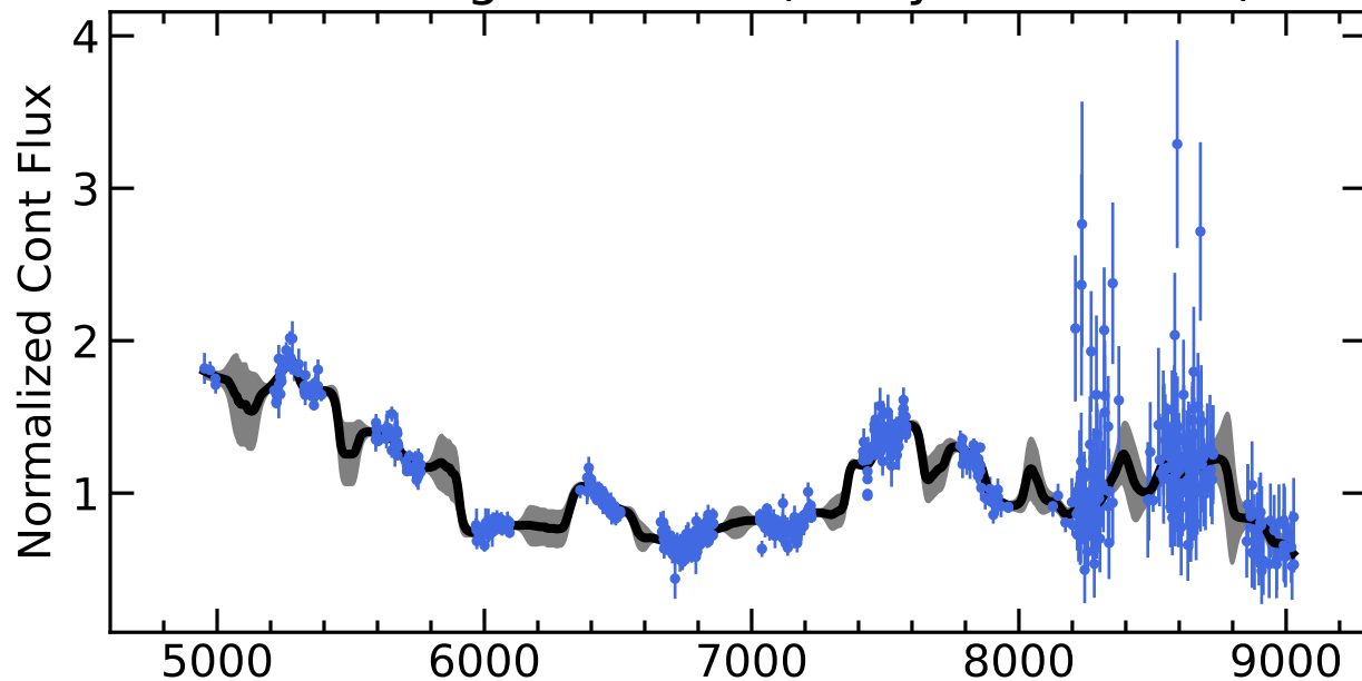
RM194 Light Curves (w/ PyROA model)
