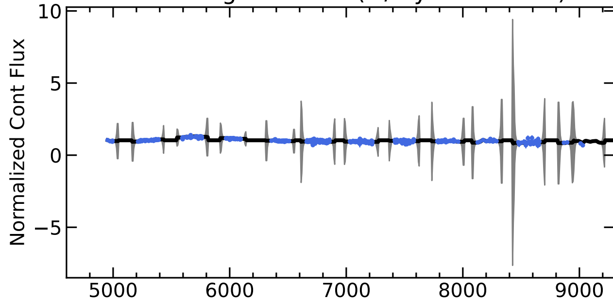
RM195 Light Curves (w/ PyROA model)
