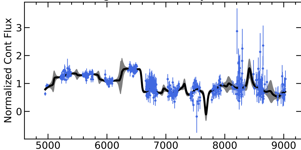
RM196 Light Curves (w/ PyROA model)
