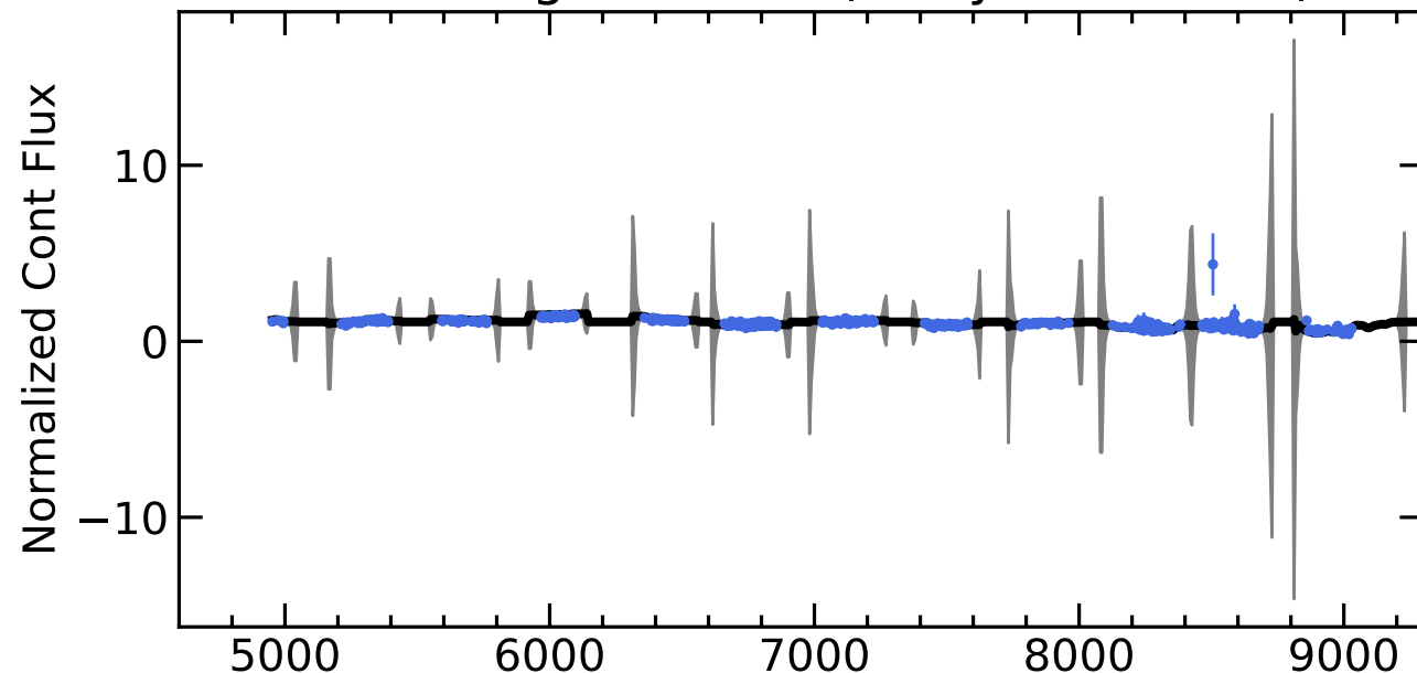
RM198 Light Curves (w/ PyROA model)
