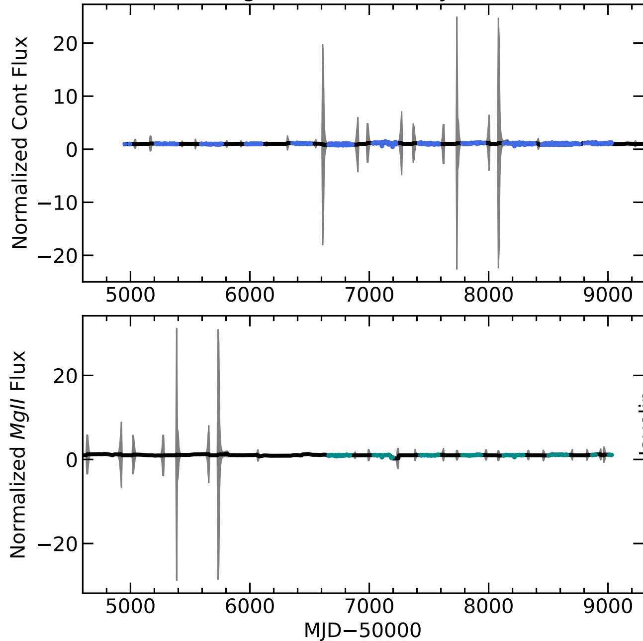
RM201 Light Curves (w/ PyROA model)
