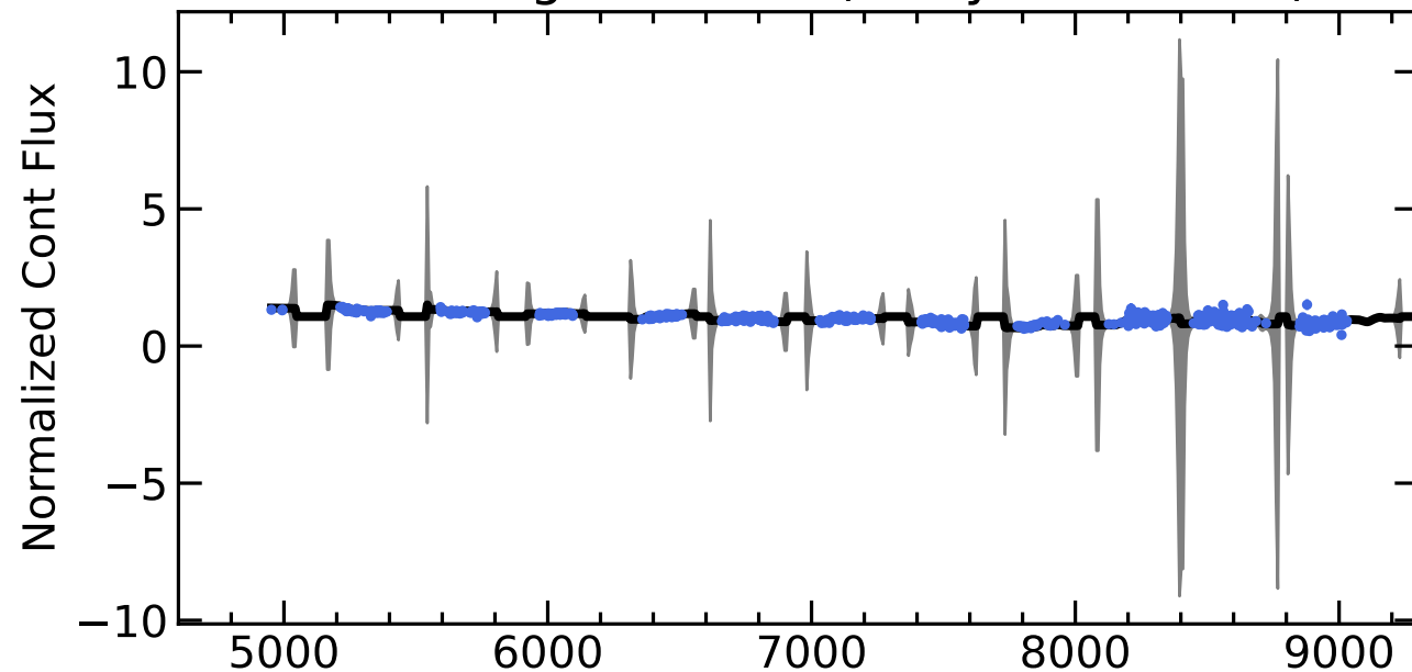
RM202 Light Curves (w/ PyROA model)
