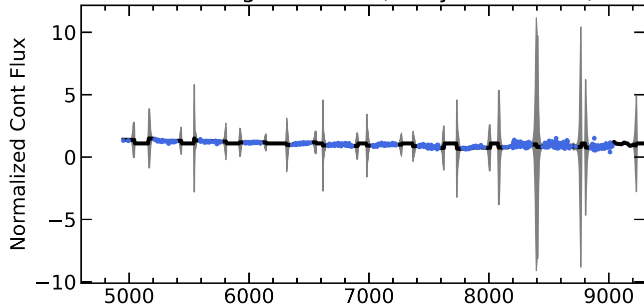
RM202 Light Curves (w/ PyROA model)
