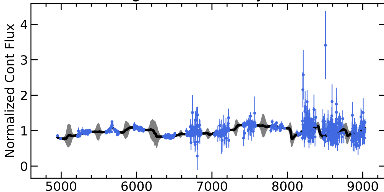
RM203 Light Curves (w/ PyROA model)
