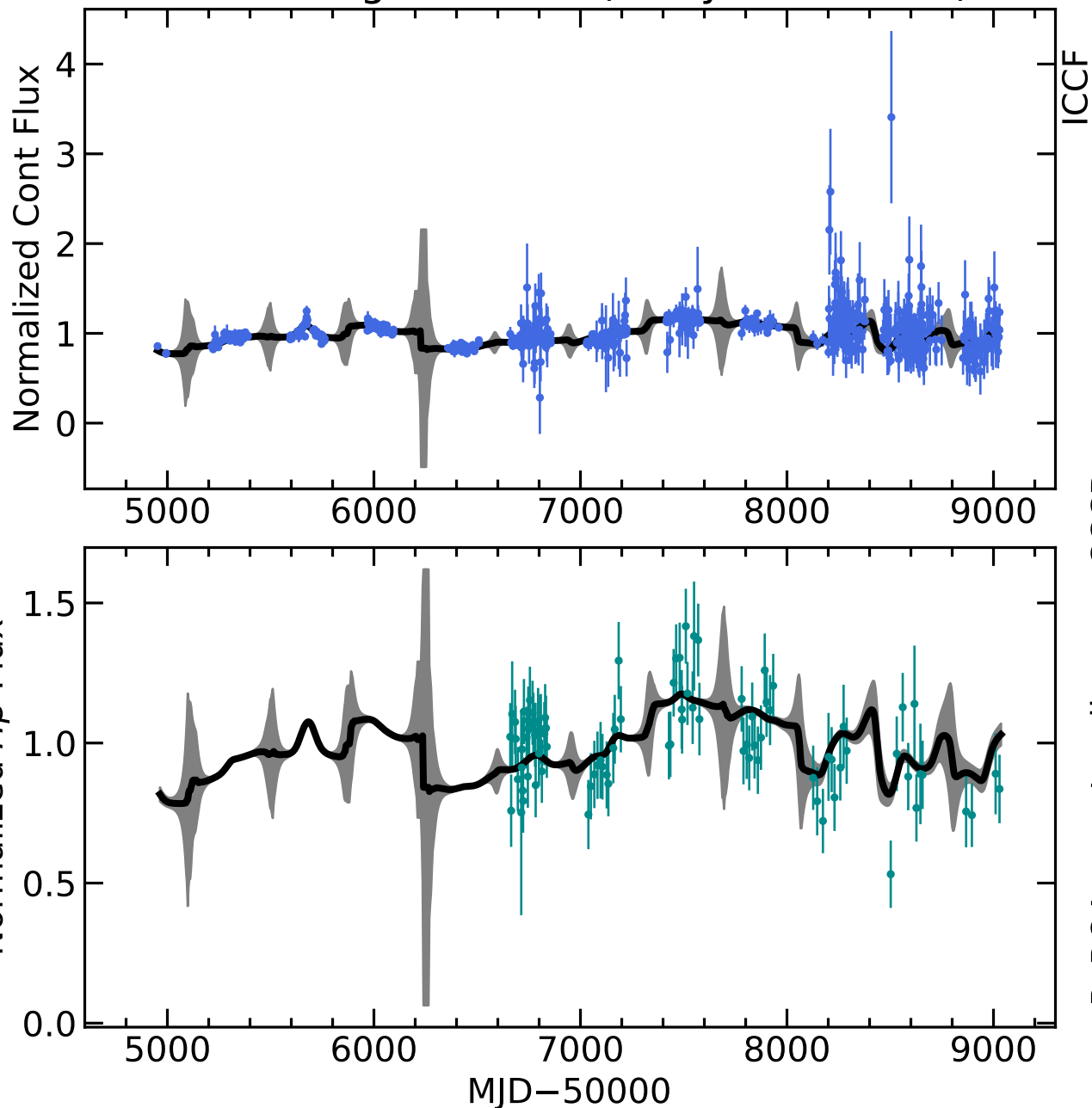
RM203 Light Curves (w/ PyROA model)
