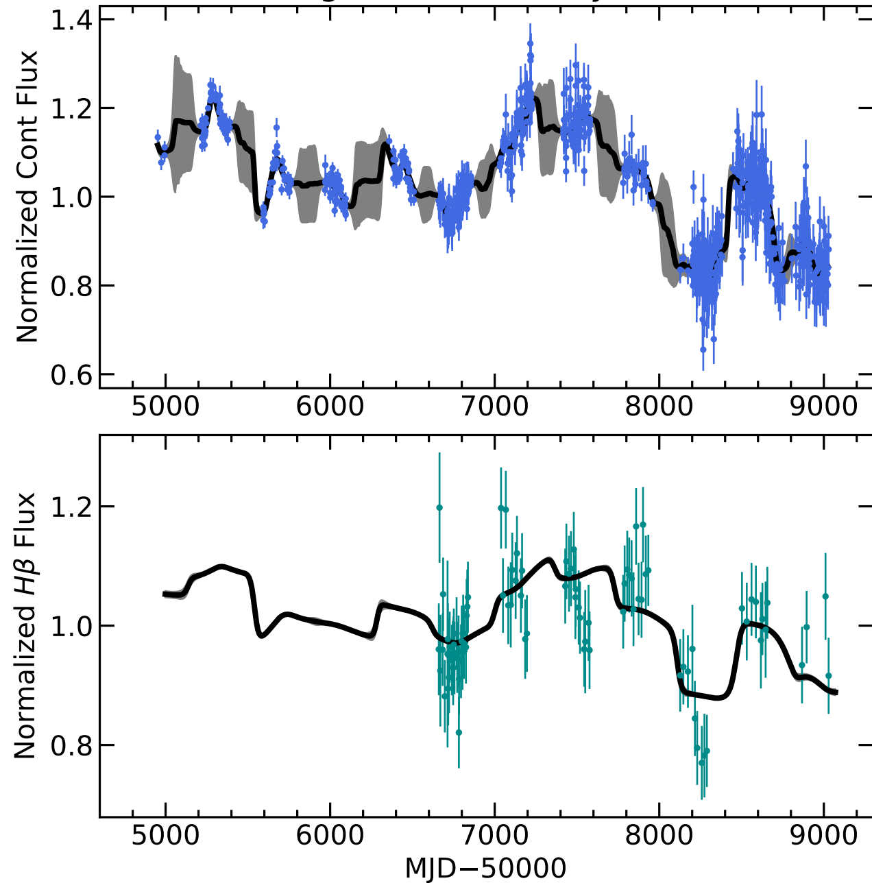
RM204 Light Curves (w/ PyROA model)
