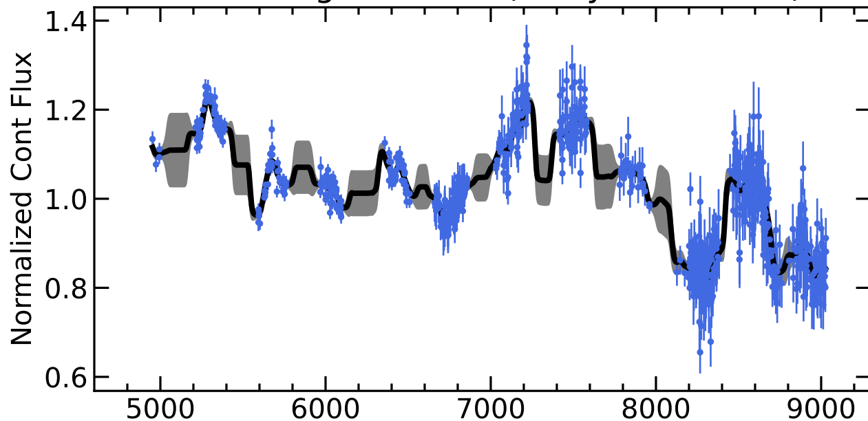
RM204 Light Curves (w/ PyROA model)
