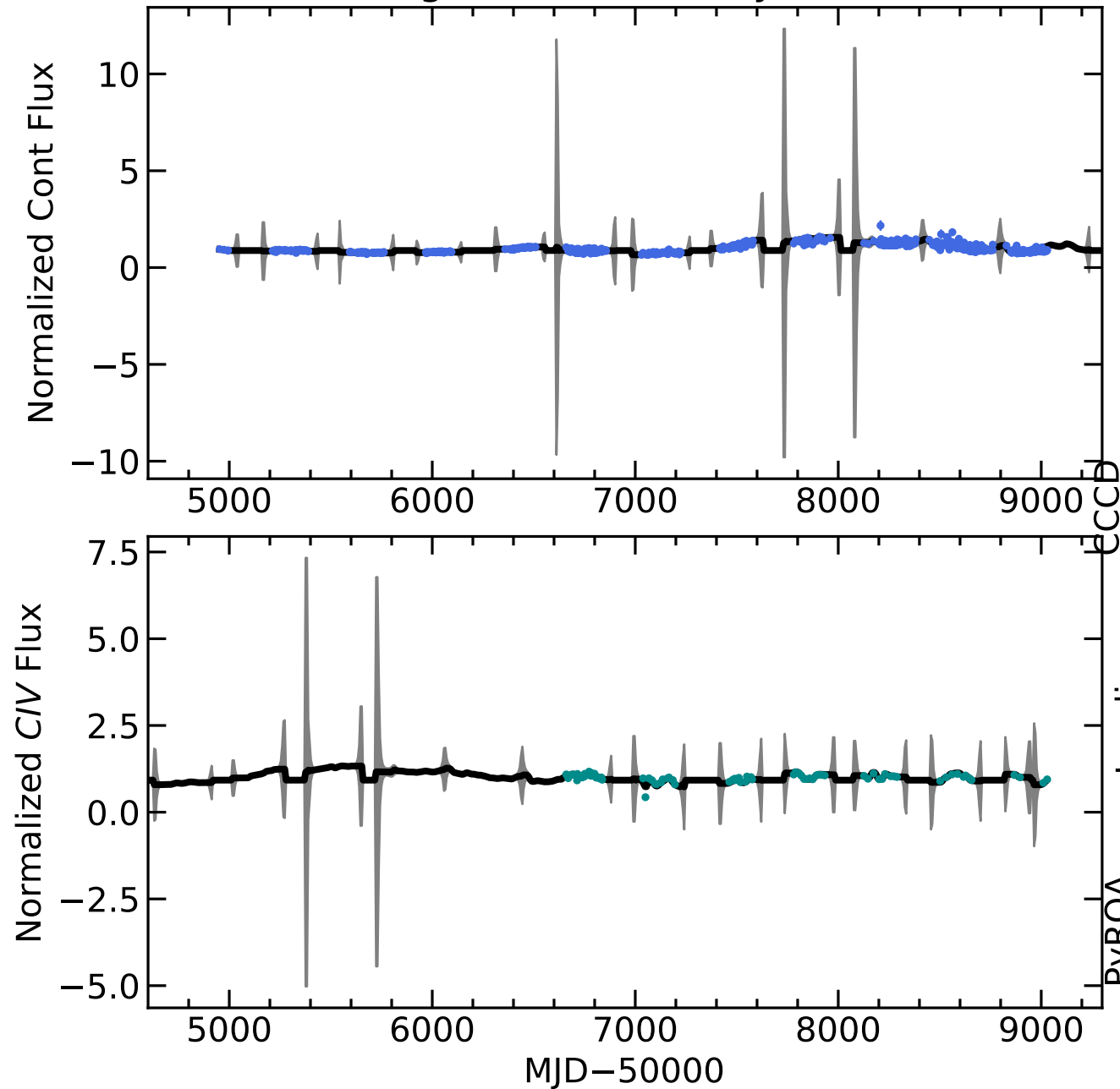
RM205 Light Curves (w/ PyROA model)
