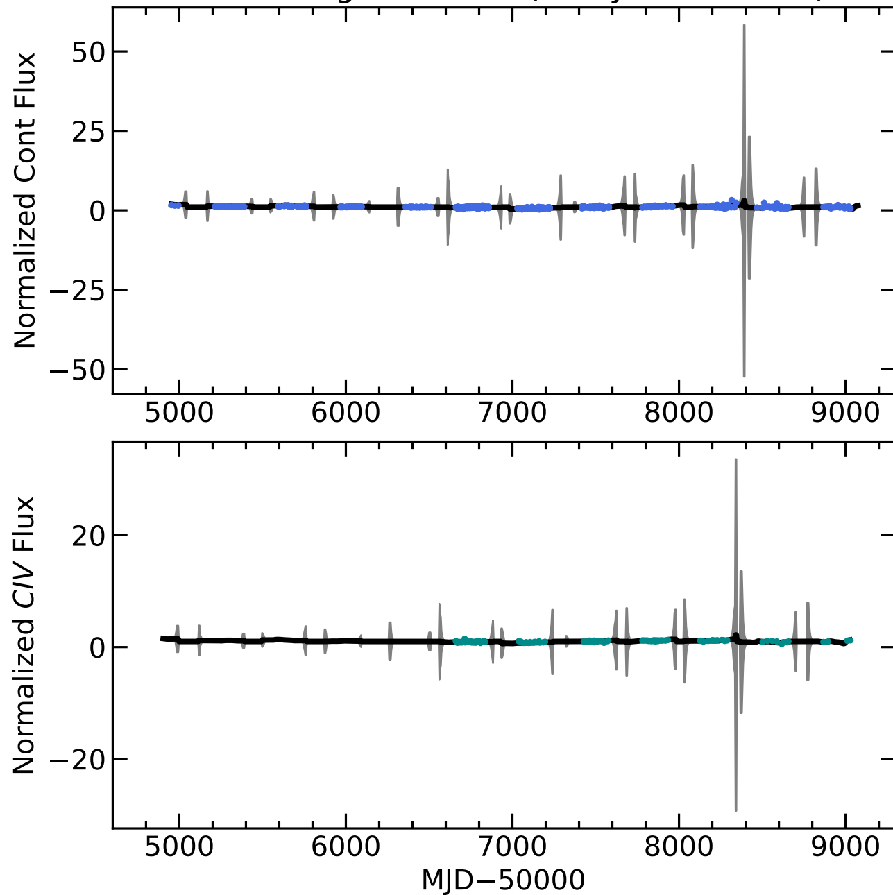
RM206 Light Curves (w/ PyROA model)
