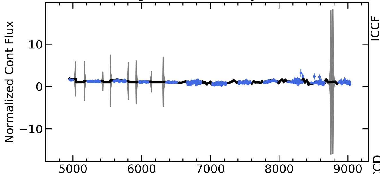
RM206 Light Curves (w/ PyROA model)
