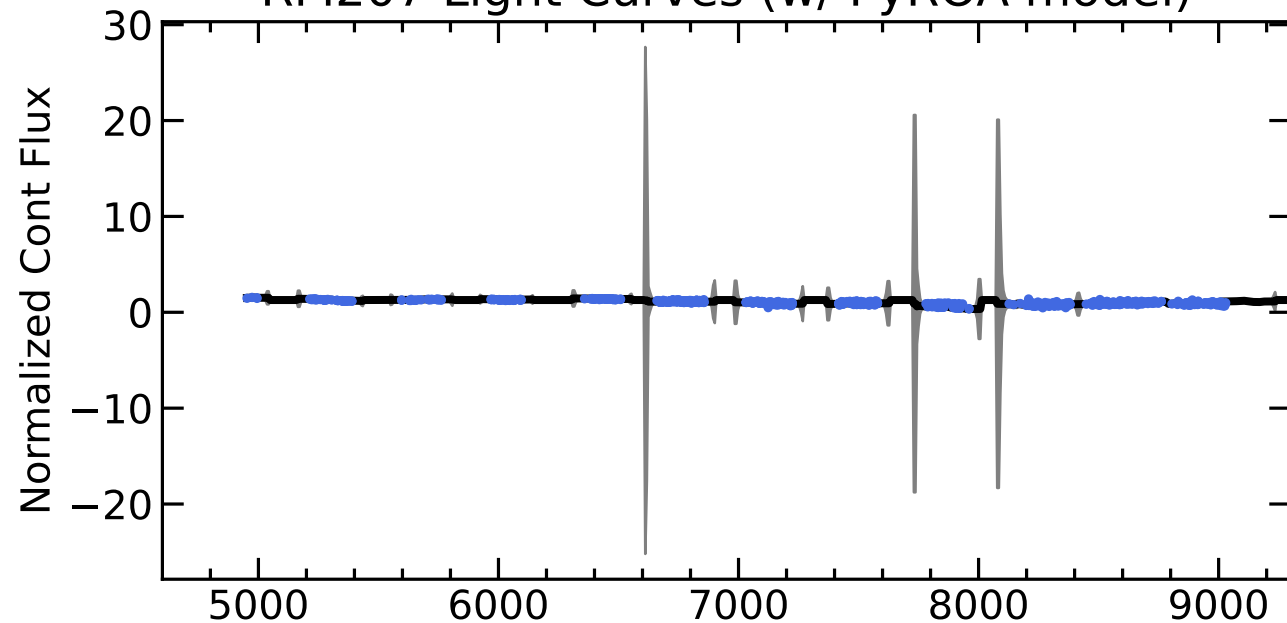
RM207 Light Curves (w/ PyROA model)
