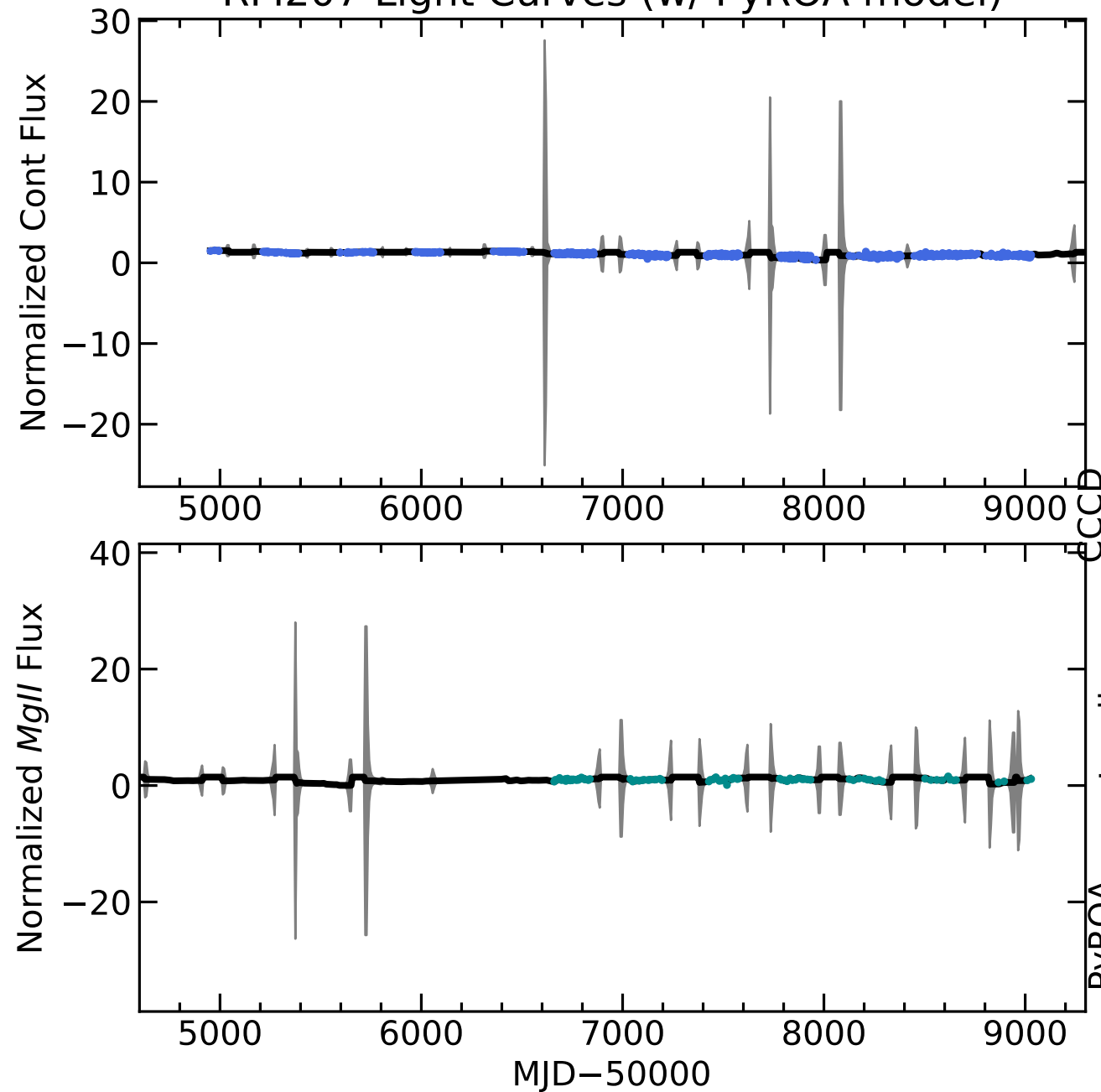
RM207 Light Curves (w/ PyROA model)
